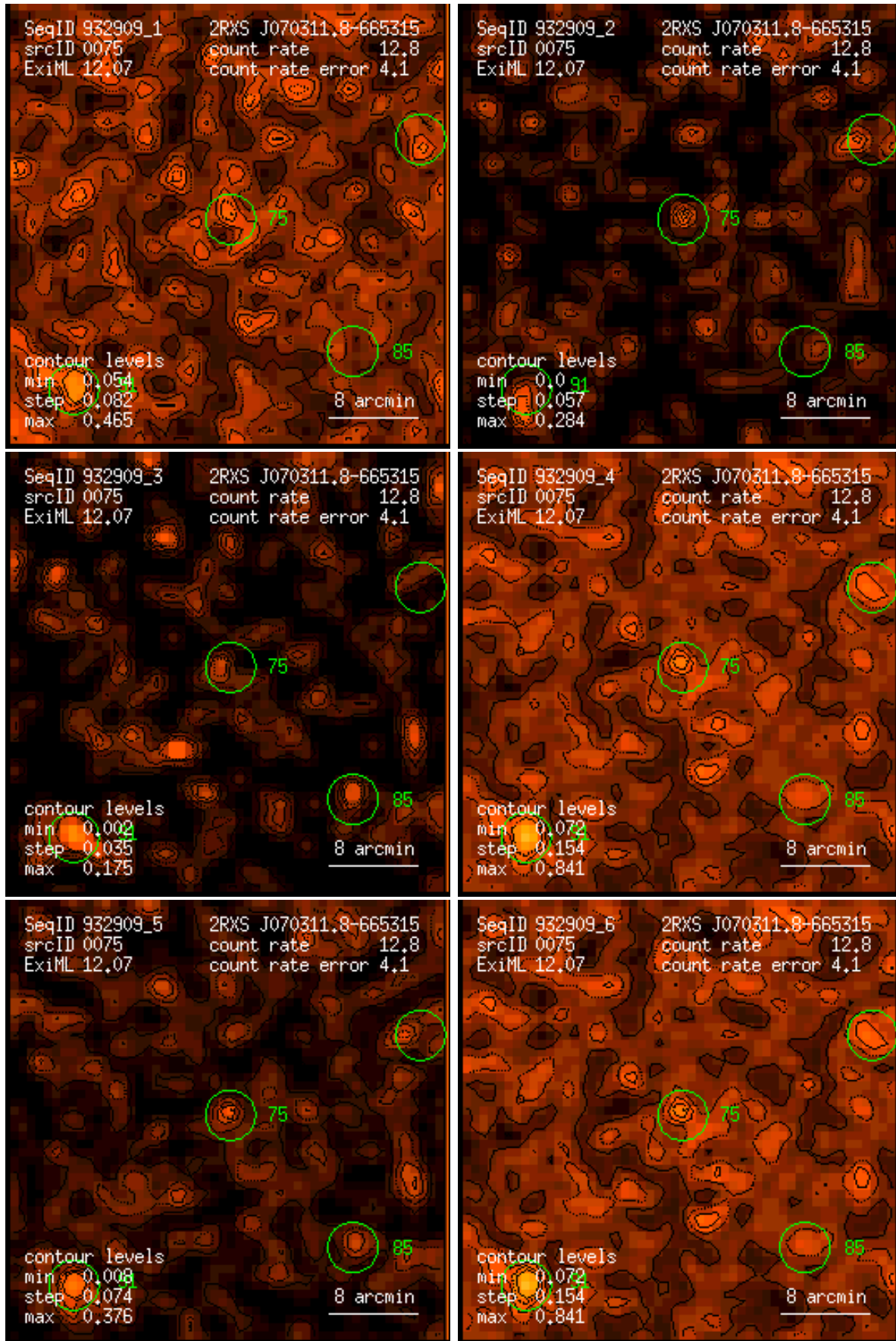
Figure 75: RASS 932909: detection 0075: band rate images, Gaussian filter: (1) PSPC channels 11 – 41, (2) 52 – 90, (3) 91 – 201, (4) 11 – 235, (5) 52 – 201, (6) 11 – 201. Broad band rates in counts/ks. Band rate contour levels in counts/ks/arcmin 2 .
