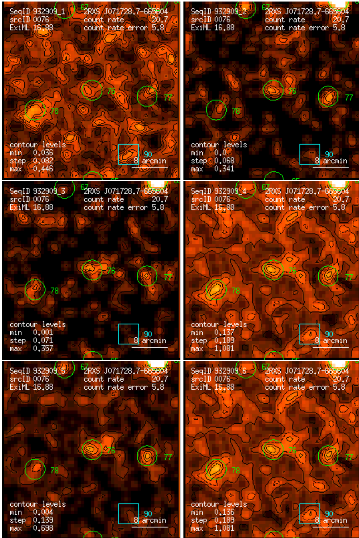
Figure 76: RASS 932909: detection 0076: band rate images, Gaussian filter: (1) PSPC channels 11 – 41, (2) 52 – 90, (3) 91 – 201, (4) 11 – 235, (5) 52 – 201, (6) 11 – 201. Broad band rates in counts/ks. Band rate contour levels in counts/ks/arcmin 2 .
