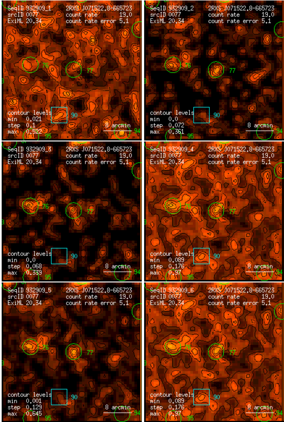
Figure 77: RASS 932909: detection 0077: band rate images, Gaussian filter: (1) PSPC channels 11 – 41, (2) 52 – 90, (3) 91 – 201, (4) 11 – 235, (5) 52 – 201, (6) 11 – 201. Broad band rates in counts/ks. Band rate contour levels in counts/ks/arcmin 2 .
