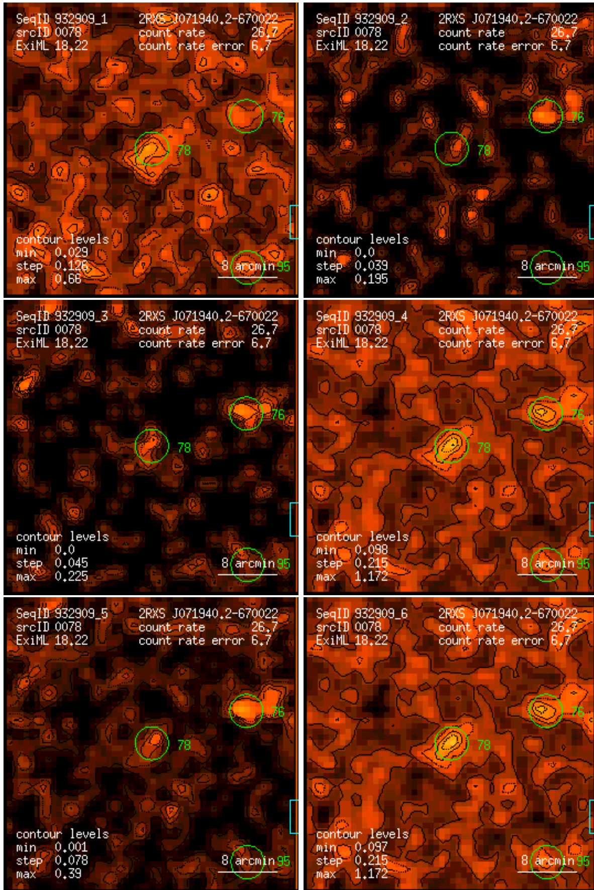
Figure 78: RASS 932909: detection 0078: band rate images, Gaussian filter: (1) PSPC channels 11 – 41, (2) 52 – 90, (3) 91 – 201, (4) 11 – 235, (5) 52 – 201, (6) 11 – 201. Broad band rates in counts/ks. Band rate contour levels in counts/ks/arcmin 2 .
