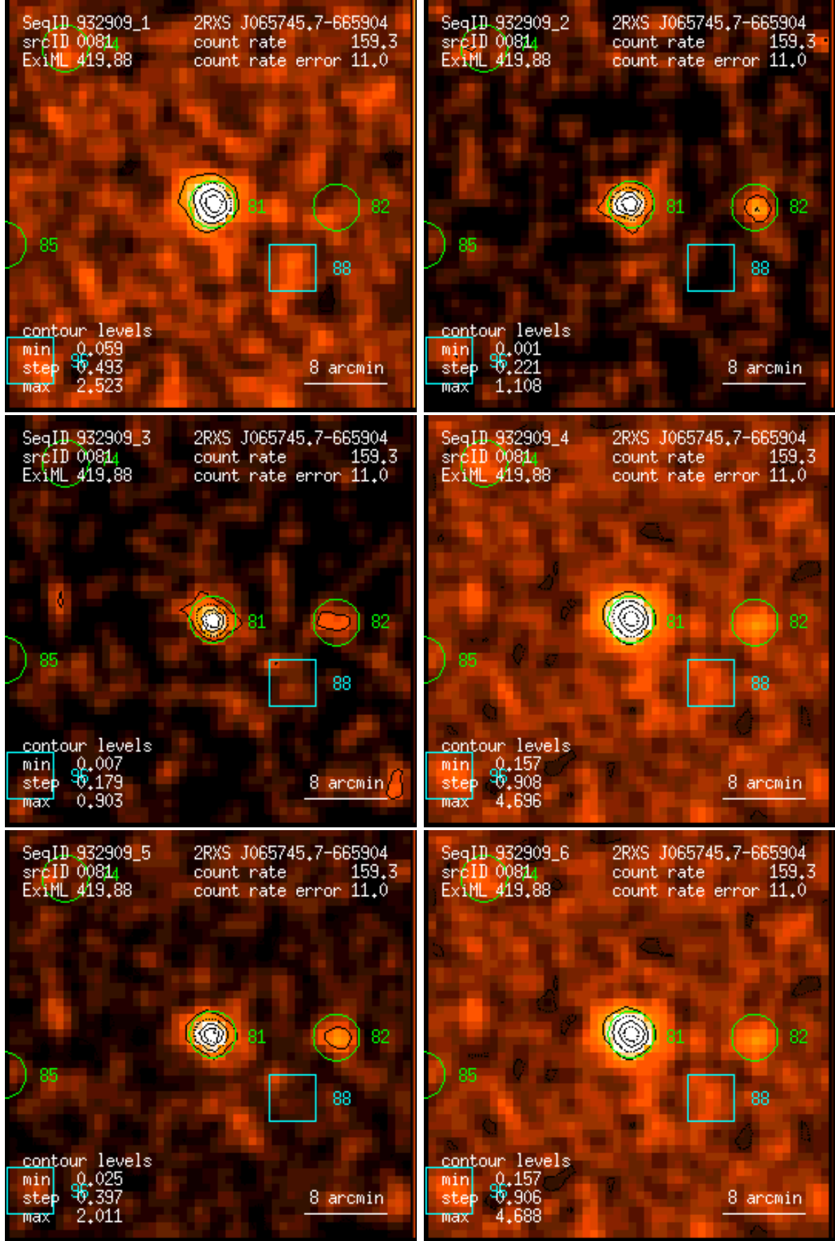
Figure 81: RASS 932909: detection 0081: band rate images, Gaussian filter: (1) PSPC channels 11 – 41, (2) 52 – 90, (3) 91 – 201, (4) 11 – 235, (5) 52 – 201, (6) 11 – 201. Broad band rates in counts/ks. Band rate contour levels in counts/ks/arcmin 2 .
