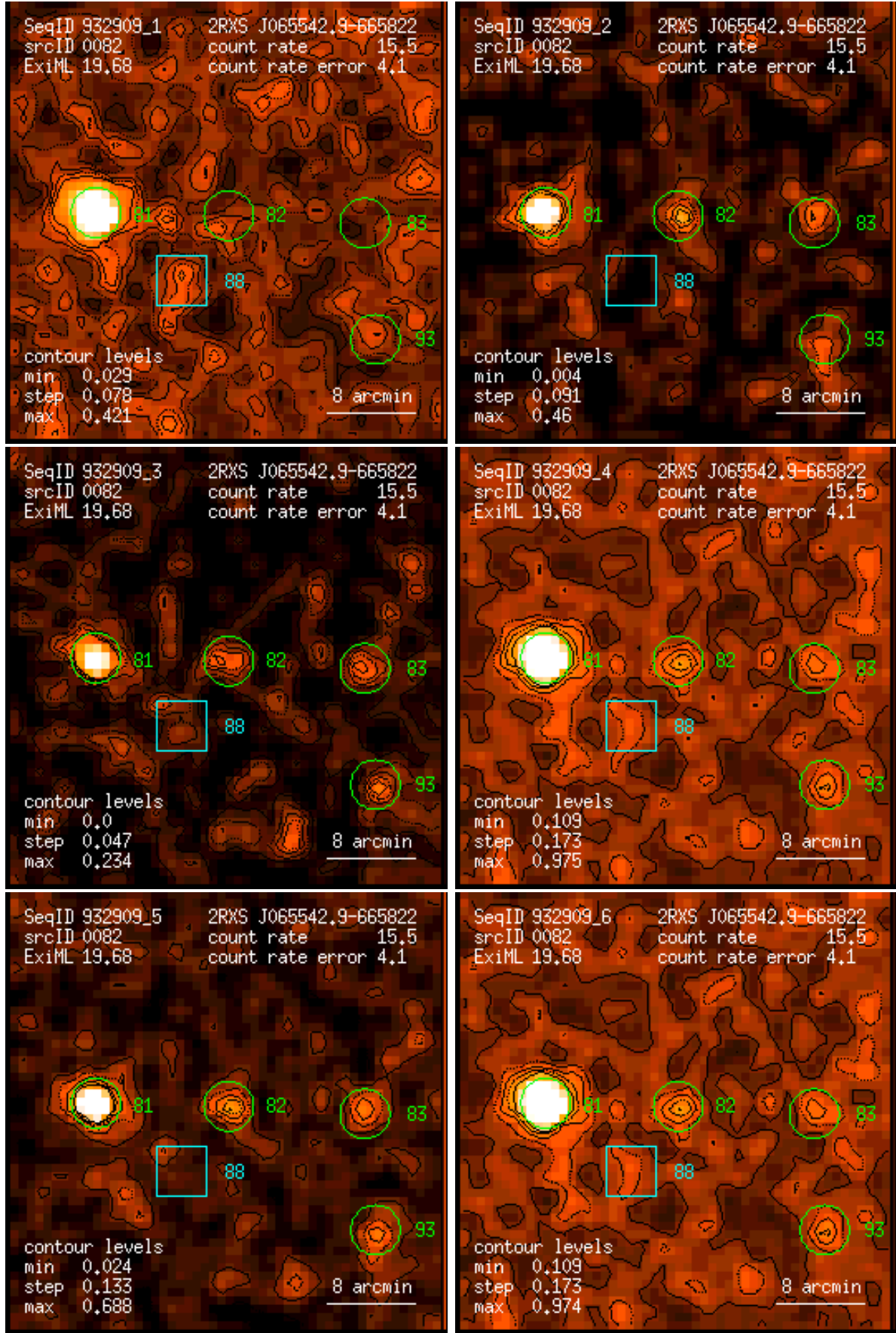
Figure 82: RASS 932909: detection 0082: band rate images, Gaussian filter: (1) PSPC channels 11 – 41, (2) 52 – 90, (3) 91 – 201, (4) 11 – 235, (5) 52 – 201, (6) 11 – 201. Broad band rates in counts/ks. Band rate contour levels in counts/ks/arcmin 2 .
