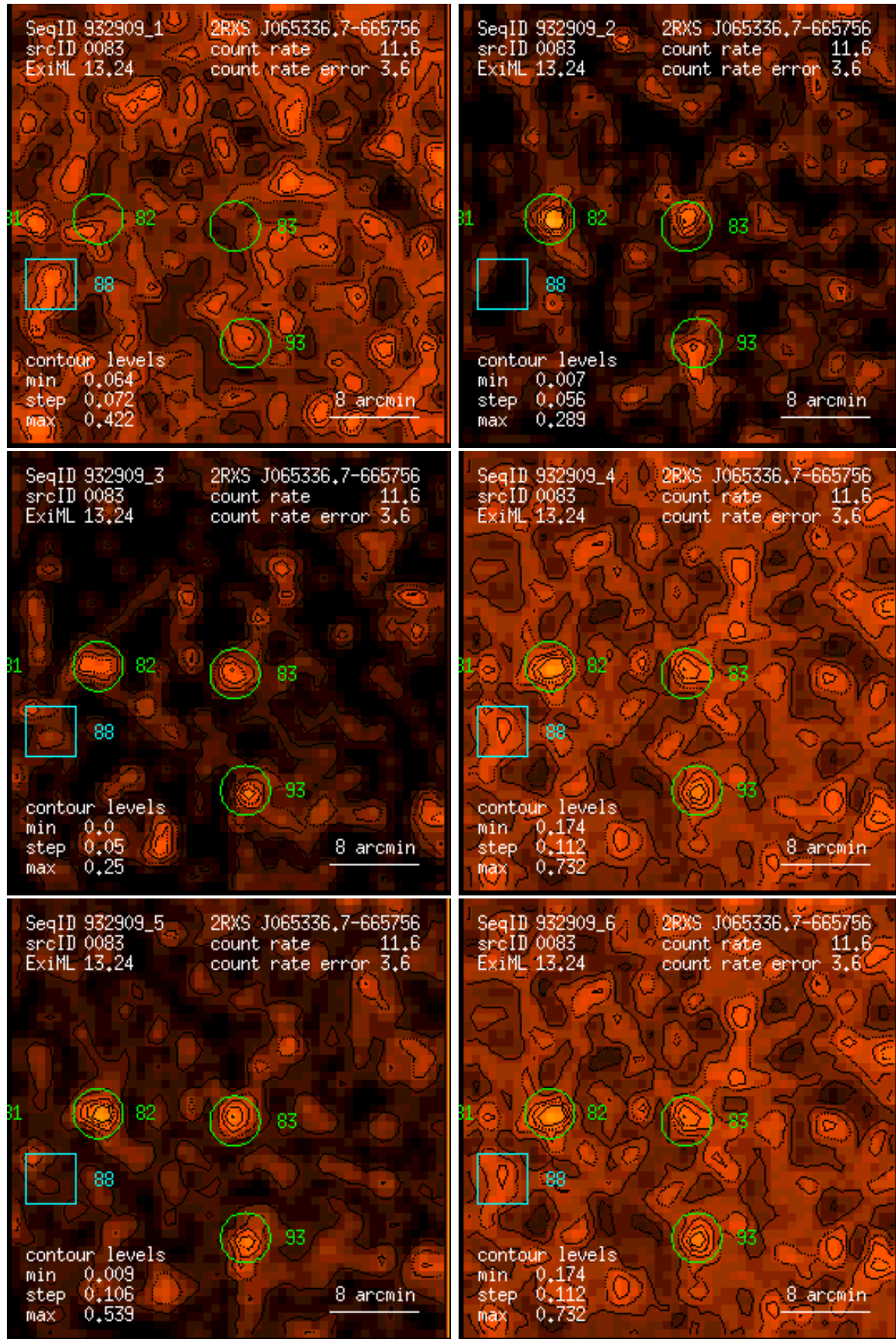
Figure 83: RASS 932909: detection 0083: band rate images, Gaussian filter: (1) PSPC channels 11 – 41, (2) 52 – 90, (3) 91 – 201, (4) 11 – 235, (5) 52 – 201, (6) 11 – 201. Broad band rates in counts/ks. Band rate contour levels in counts/ks/arcmin 2 .
