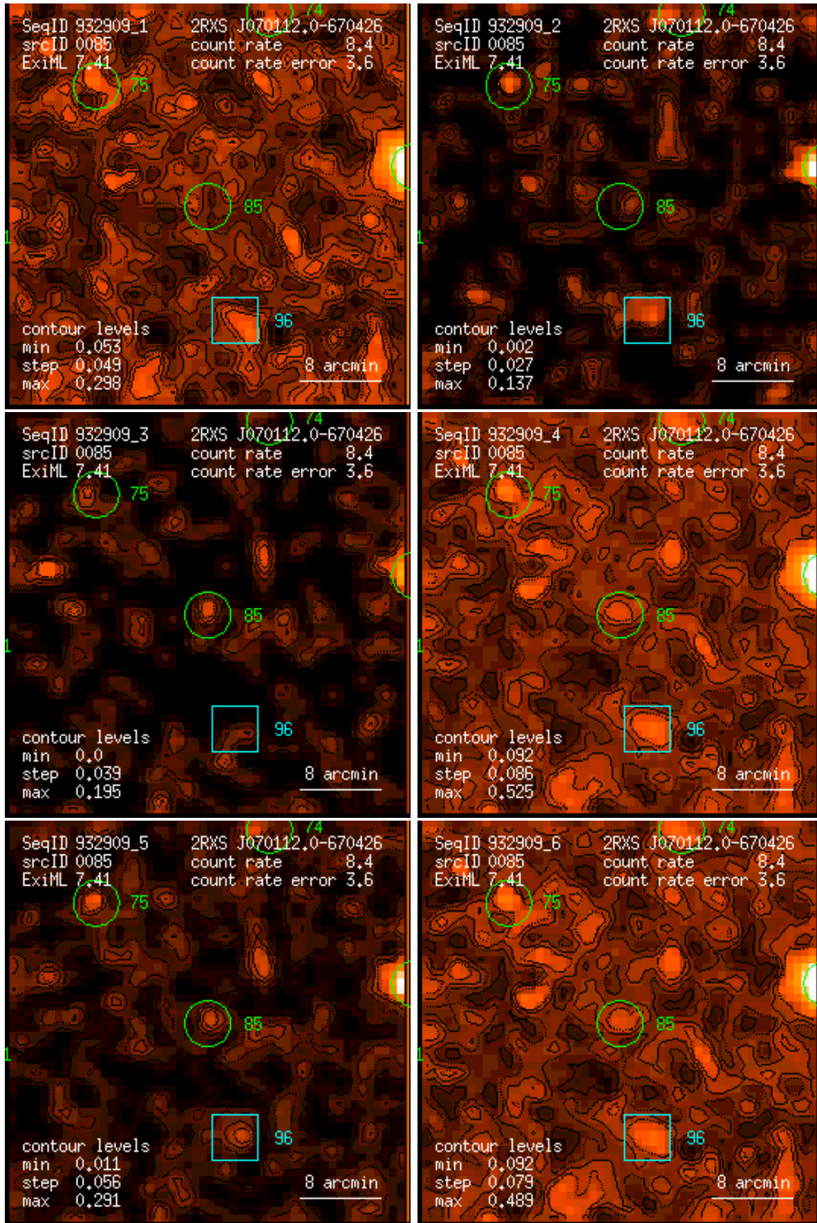
Figure 85: RASS 932909: detection 0085: band rate images, Gaussian filter: (1) PSPC channels 11 – 41, (2) 52 – 90, (3) 91 – 201, (4) 11 – 235, (5) 52 – 201, (6) 11 – 201. Broad band rates in counts/ks. Band rate contour levels in counts/ks/arcmin 2 .
