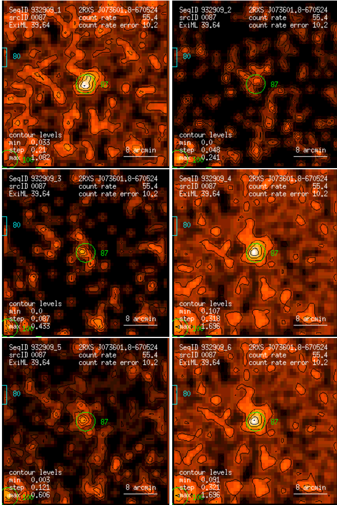
Figure 87: RASS 932909: detection 0087: band rate images, Gaussian filter: (1) PSPC channels 11 – 41, (2) 52 – 90, (3) 91 – 201, (4) 11 – 235, (5) 52 – 201, (6) 11 – 201. Broad band rates in counts/ks. Band rate contour levels in counts/ks/arcmin 2 .
