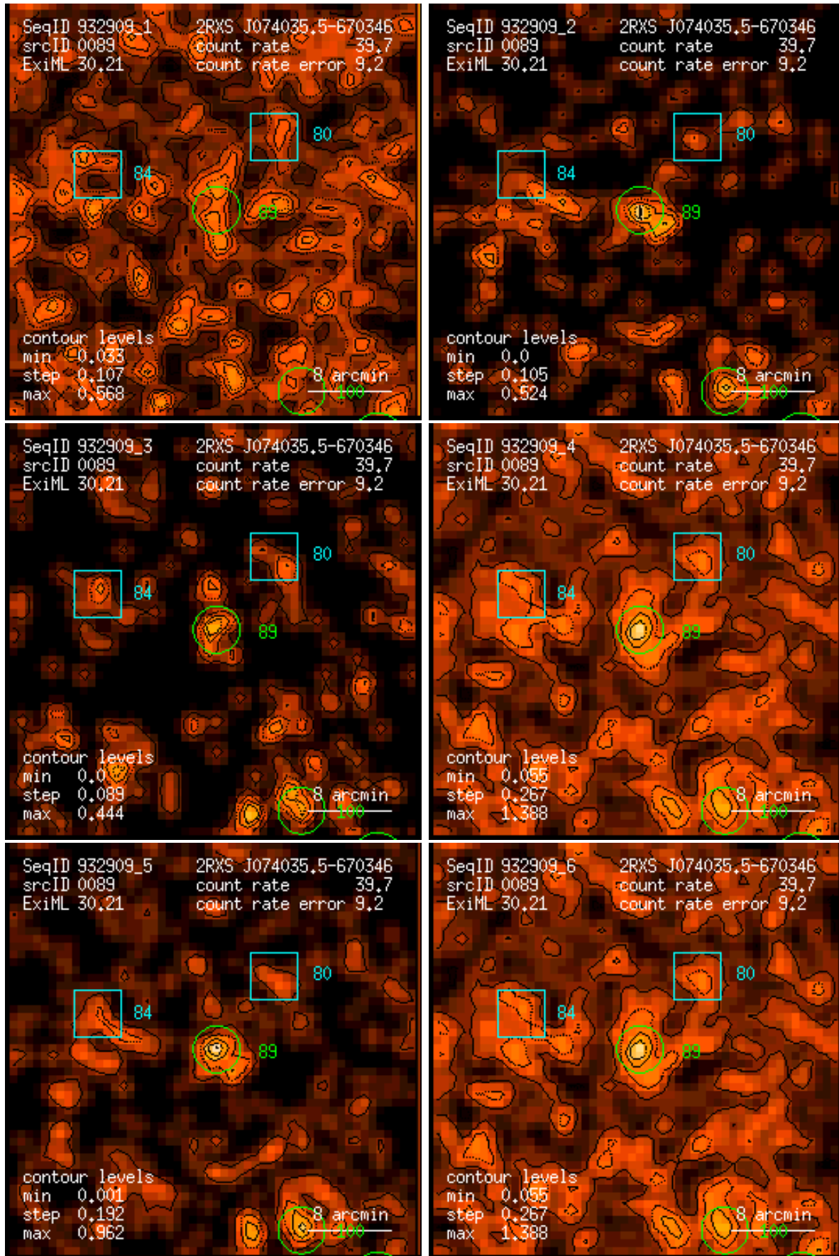
Figure 89: RASS 932909: detection 0089: band rate images, Gaussian filter: (1) PSPC channels 11 – 41, (2) 52 – 90, (3) 91 – 201, (4) 11 – 235, (5) 52 – 201, (6) 11 – 201. Broad band rates in counts/ks. Band rate contour levels in counts/ks/arcmin 2 .
