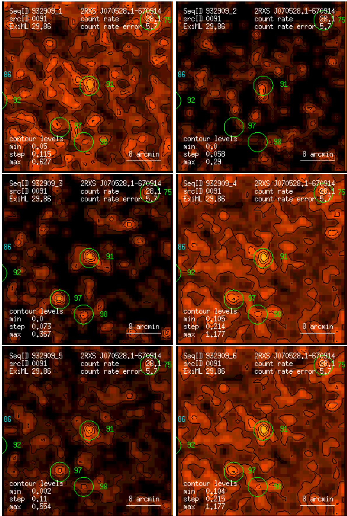
Figure 91: RASS 932909: detection 0091: band rate images, Gaussian filter: (1) PSPC channels 11 – 41, (2) 52 – 90, (3) 91 – 201, (4) 11 – 235, (5) 52 – 201, (6) 11 – 201. Broad band rates in counts/ks. Band rate contour levels in counts/ks/arcmin 2 .
