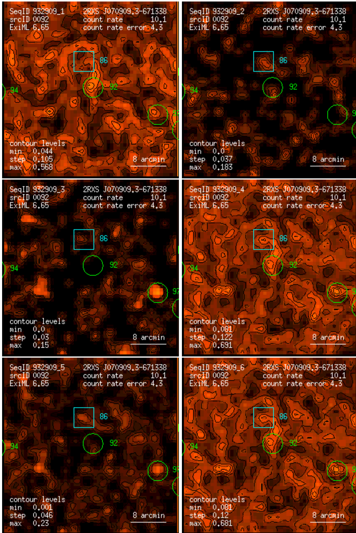
Figure 92: RASS 932909: detection 0092: band rate images, Gaussian filter: (1) PSPC channels 11 – 41, (2) 52 – 90, (3) 91 – 201, (4) 11 – 235, (5) 52 – 201, (6) 11 – 201. Broad band rates in counts/ks. Band rate contour levels in counts/ks/arcmin 2 .
