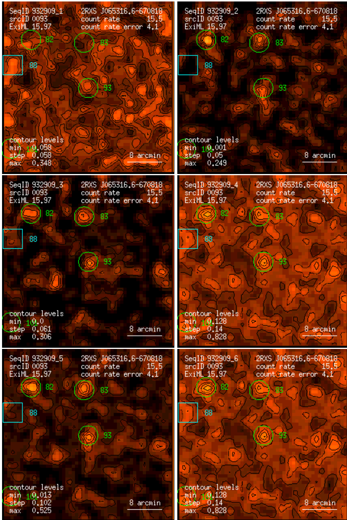
Figure 93: RASS 932909: detection 0093: band rate images, Gaussian filter: (1) PSPC channels 11 – 41, (2) 52 – 90, (3) 91 – 201, (4) 11 – 235, (5) 52 – 201, (6) 11 – 201. Broad band rates in counts/ks. Band rate contour levels in counts/ks/arcmin 2 .
