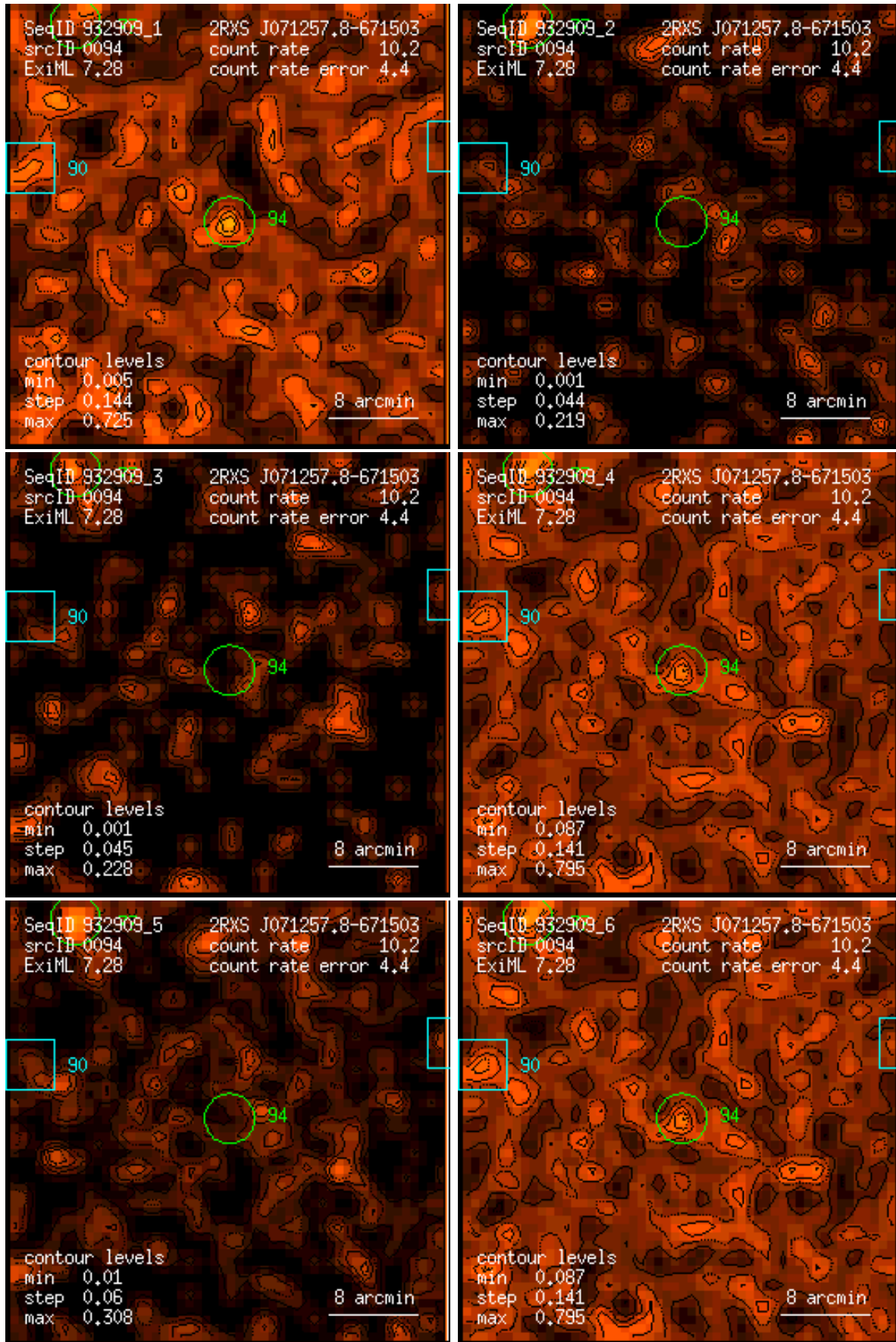
Figure 94: RASS 932909: detection 0094: band rate images, Gaussian filter: (1) PSPC channels 11 – 41, (2) 52 – 90, (3) 91 – 201, (4) 11 – 235, (5) 52 – 201, (6) 11 – 201. Broad band rates in counts/ks. Band rate contour levels in counts/ks/arcmin 2 .
