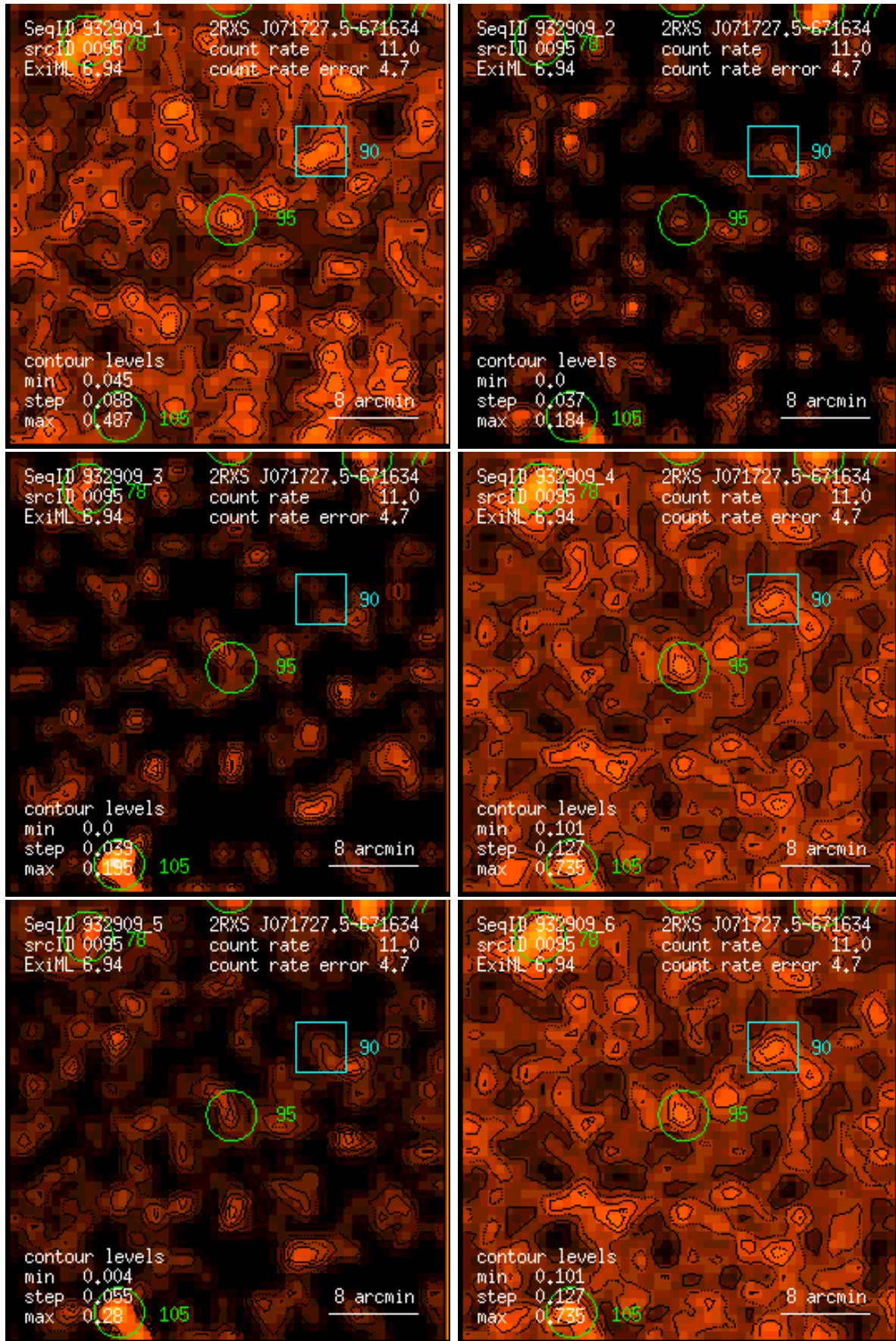
Figure 95: RASS 932909: detection 0095: band rate images, Gaussian filter: (1) PSPC channels 11 – 41, (2) 52 – 90, (3) 91 – 201, (4) 11 – 235, (5) 52 – 201, (6) 11 – 201. Broad band rates in counts/ks. Band rate contour levels in counts/ks/arcmin 2 .
