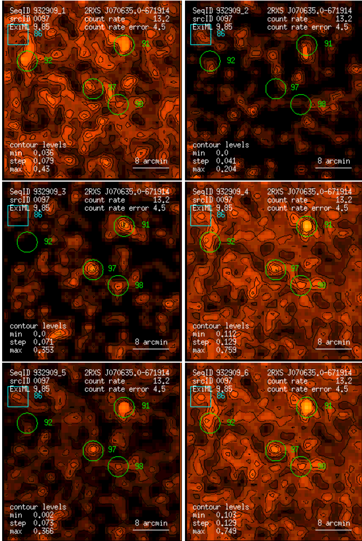
Figure 97: RASS 932909: detection 0097: band rate images, Gaussian filter: (1) PSPC channels 11 – 41, (2) 52 – 90, (3) 91 – 201, (4) 11 – 235, (5) 52 – 201, (6) 11 – 201. Broad band rates in counts/ks. Band rate contour levels in counts/ks/arcmin 2 .
