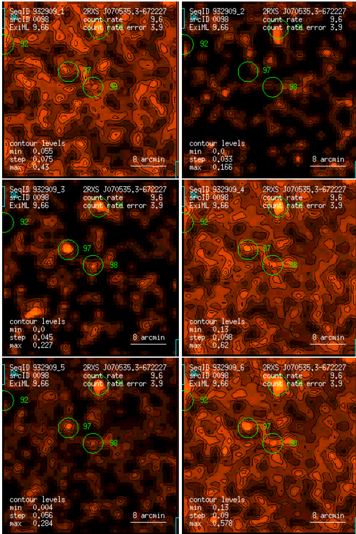
Figure 98: RASS 932909: detection 0098: band rate images, Gaussian filter: (1) PSPC channels 11 – 41, (2) 52 – 90, (3) 91 – 201, (4) 11 – 235, (5) 52 – 201, (6) 11 – 201. Broad band rates in counts/ks. Band rate contour levels in counts/ks/arcmin 2 .
