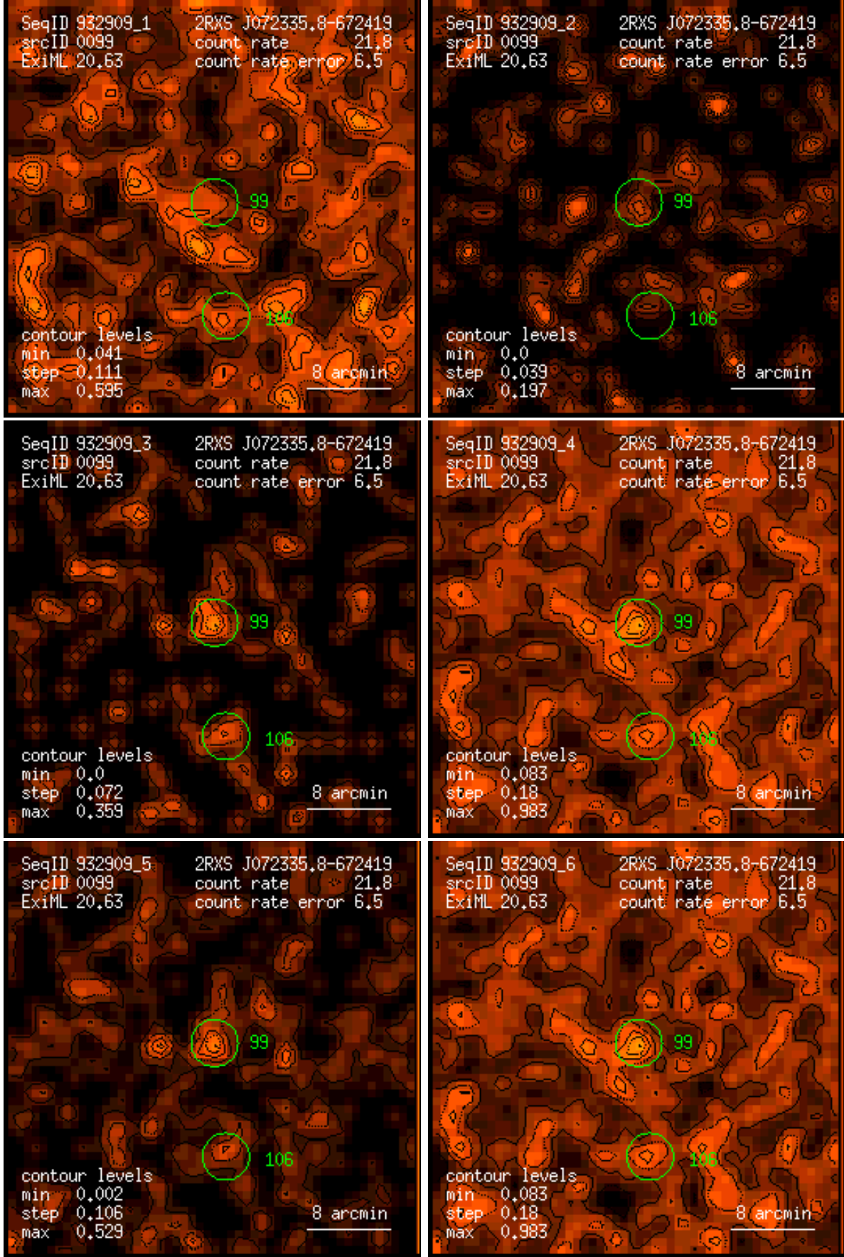
Figure 99: RASS 932909: detection 0099: band rate images, Gaussian filter: (1) PSPC channels 11 – 41, (2) 52 – 90, (3) 91 – 201, (4) 11 – 235, (5) 52 – 201, (6) 11 – 201. Broad band rates in counts/ks. Band rate contour levels in counts/ks/arcmin 2 .
