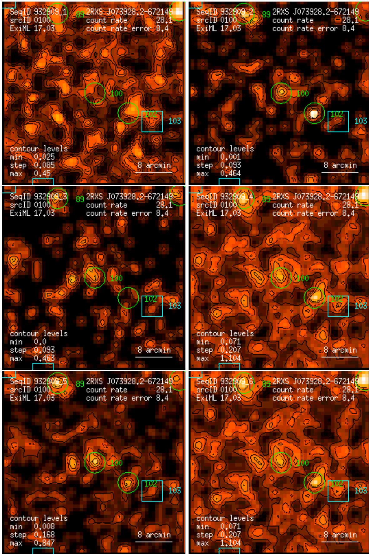
Figure 100: RASS 932909: detection 0100: band rate images, Gaussian filter: (1) PSPC channels 11 – 41, (2) 52 – 90, (3) 91 – 201, (4) 11 – 235, (5) 52 – 201, (6) 11 – 201. Broad band rates in counts/ks. Band rate contour levels in counts/ks/arcmin 2 .
