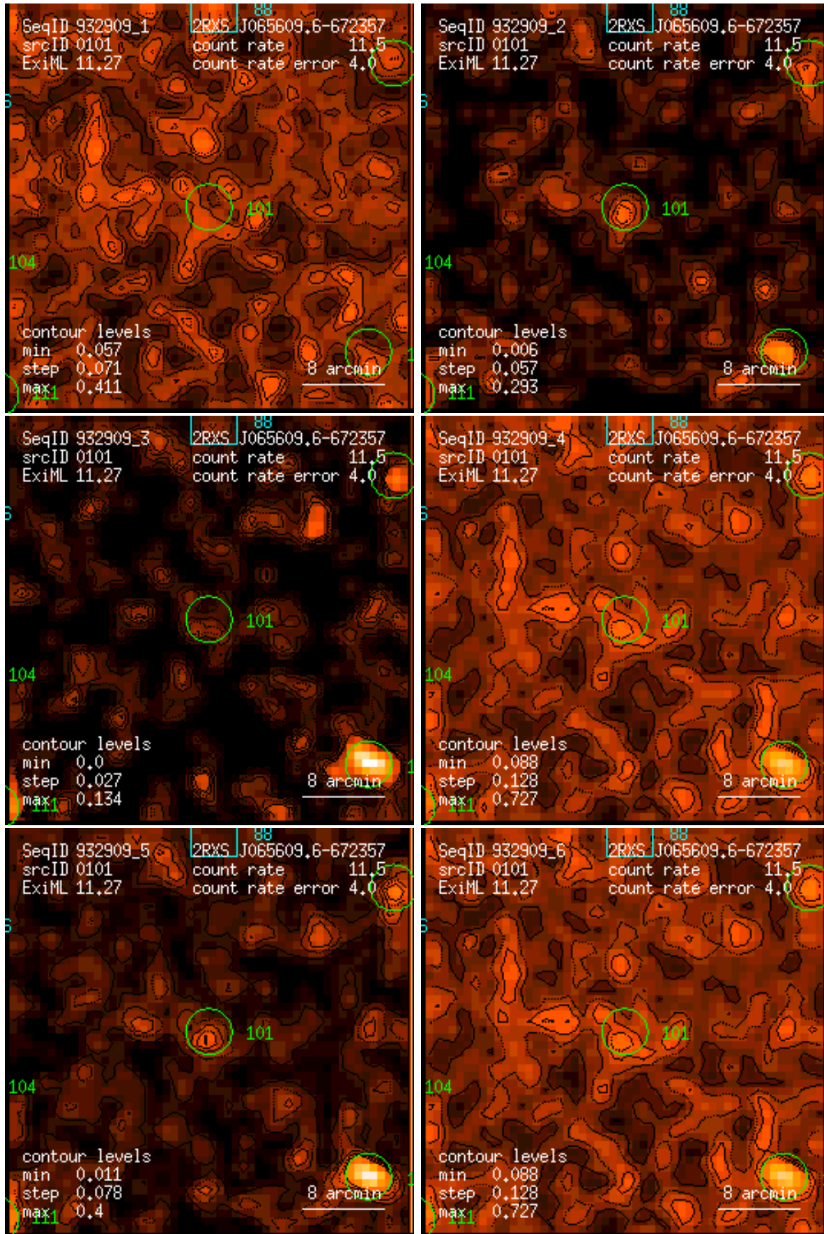
Figure 101: RASS 932909: detection 0101: band rate images, Gaussian filter: (1) PSPC channels 11 – 41, (2) 52 – 90, (3) 91 – 201, (4) 11 – 235, (5) 52 – 201, (6) 11 – 201. Broad band rates in counts/ks. Band rate contour levels in counts/ks/arcmin 2 .
