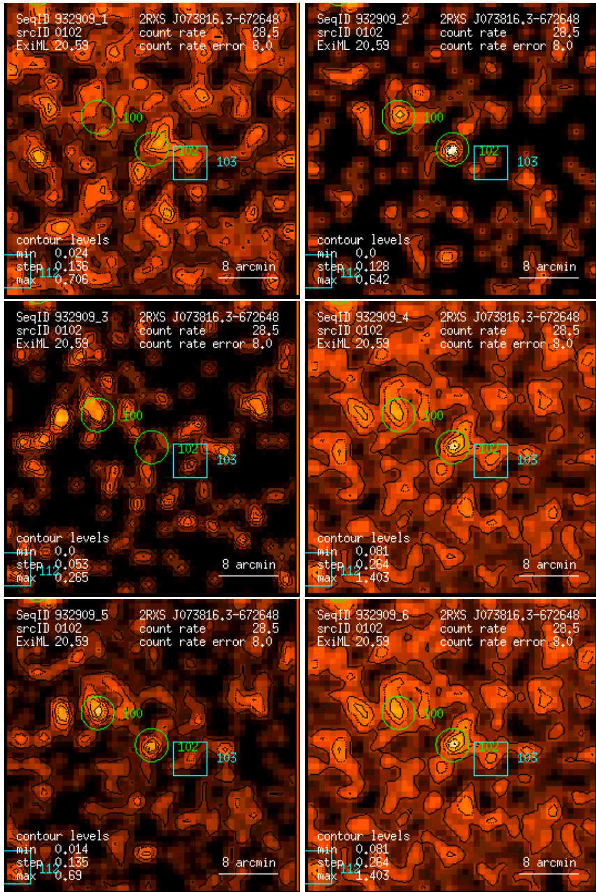
Figure 102: RASS 932909: detection 0102: band rate images, Gaussian filter: (1) PSPC channels 11 – 41, (2) 52 – 90, (3) 91 – 201, (4) 11 – 235, (5) 52 – 201, (6) 11 – 201. Broad band rates in counts/ks. Band rate contour levels in counts/ks/arcmin 2 .
