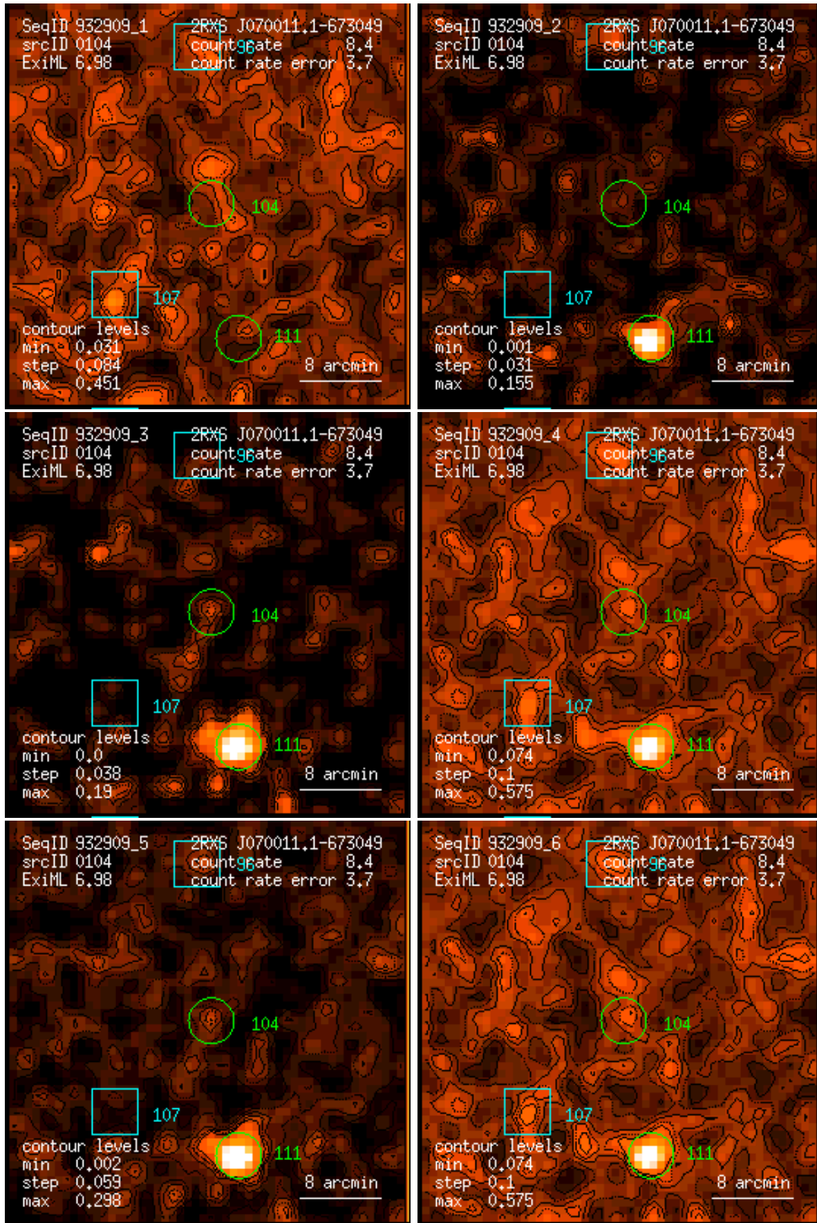
Figure 104: RASS 932909: detection 0104: band rate images, Gaussian filter: (1) PSPC channels 11 – 41, (2) 52 – 90, (3) 91 – 201, (4) 11 – 235, (5) 52 – 201, (6) 11 – 201. Broad band rates in counts/ks. Band rate contour levels in counts/ks/arcmin 2 .
