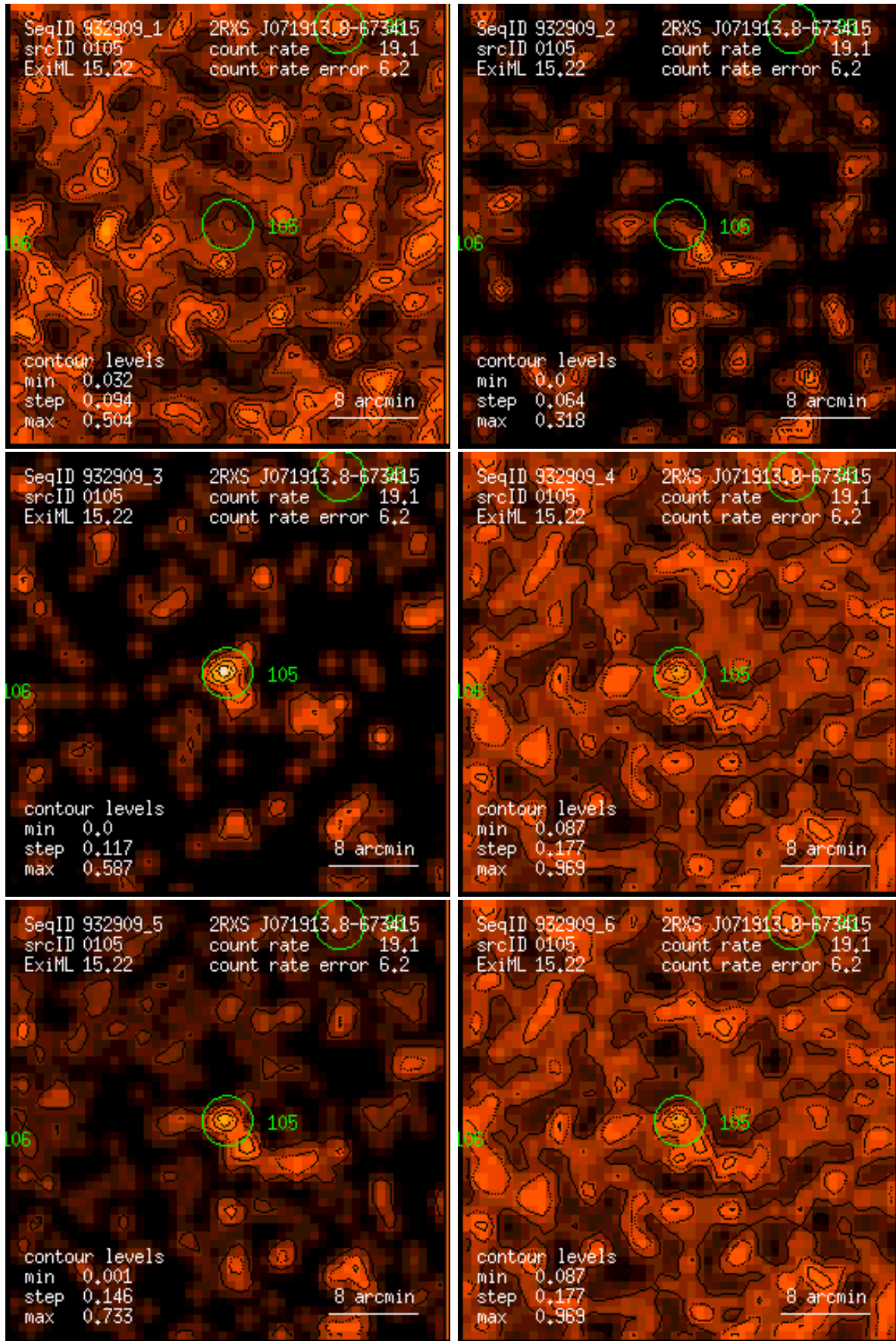
Figure 105: RASS 932909: detection 0105: band rate images, Gaussian filter: (1) PSPC channels 11 – 41, (2) 52 – 90, (3) 91 – 201, (4) 11 – 235, (5) 52 – 201, (6) 11 – 201. Broad band rates in counts/ks. Band rate contour levels in counts/ks/arcmin 2 .
