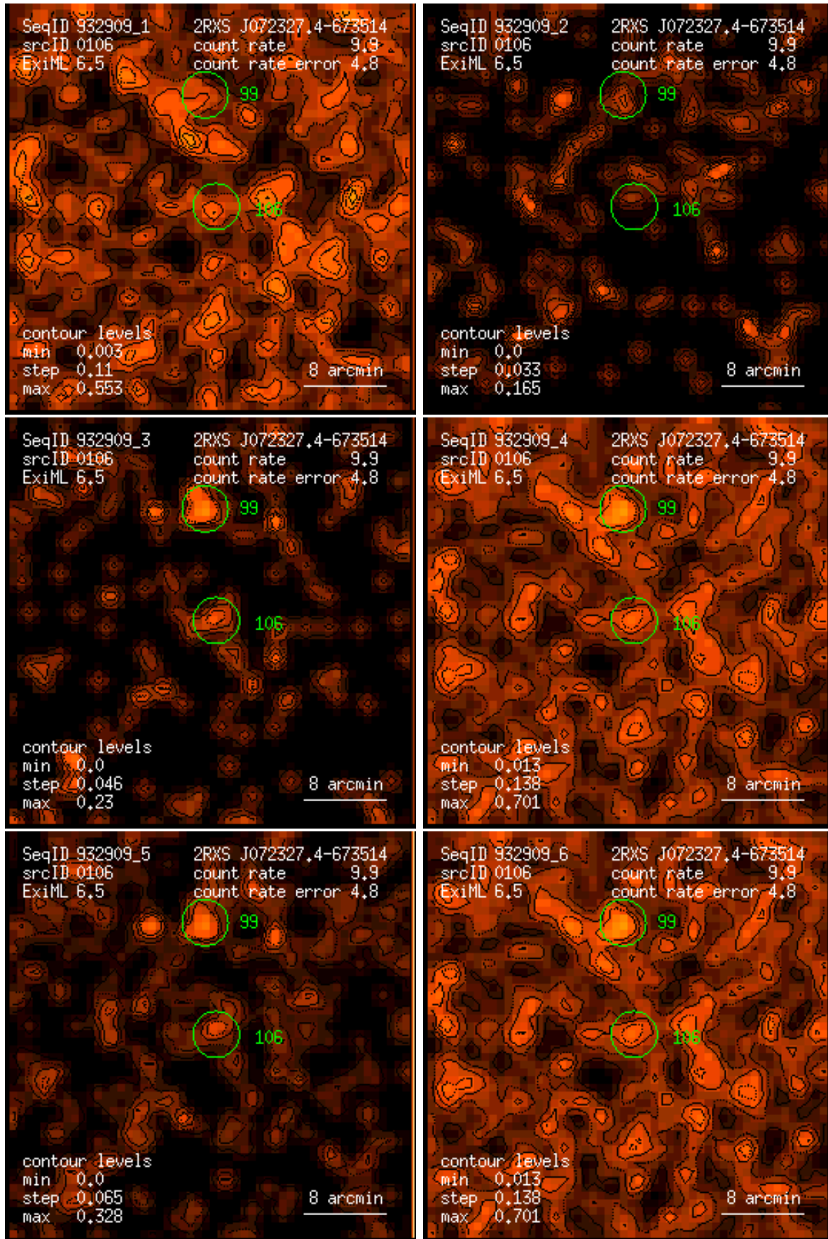
Figure 106: RASS 932909: detection 0106: band rate images, Gaussian filter: (1) PSPC channels 11 – 41, (2) 52 – 90, (3) 91 – 201, (4) 11 – 235, (5) 52 – 201, (6) 11 – 201. Broad band rates in counts/ks. Band rate contour levels in counts/ks/arcmin 2 .
