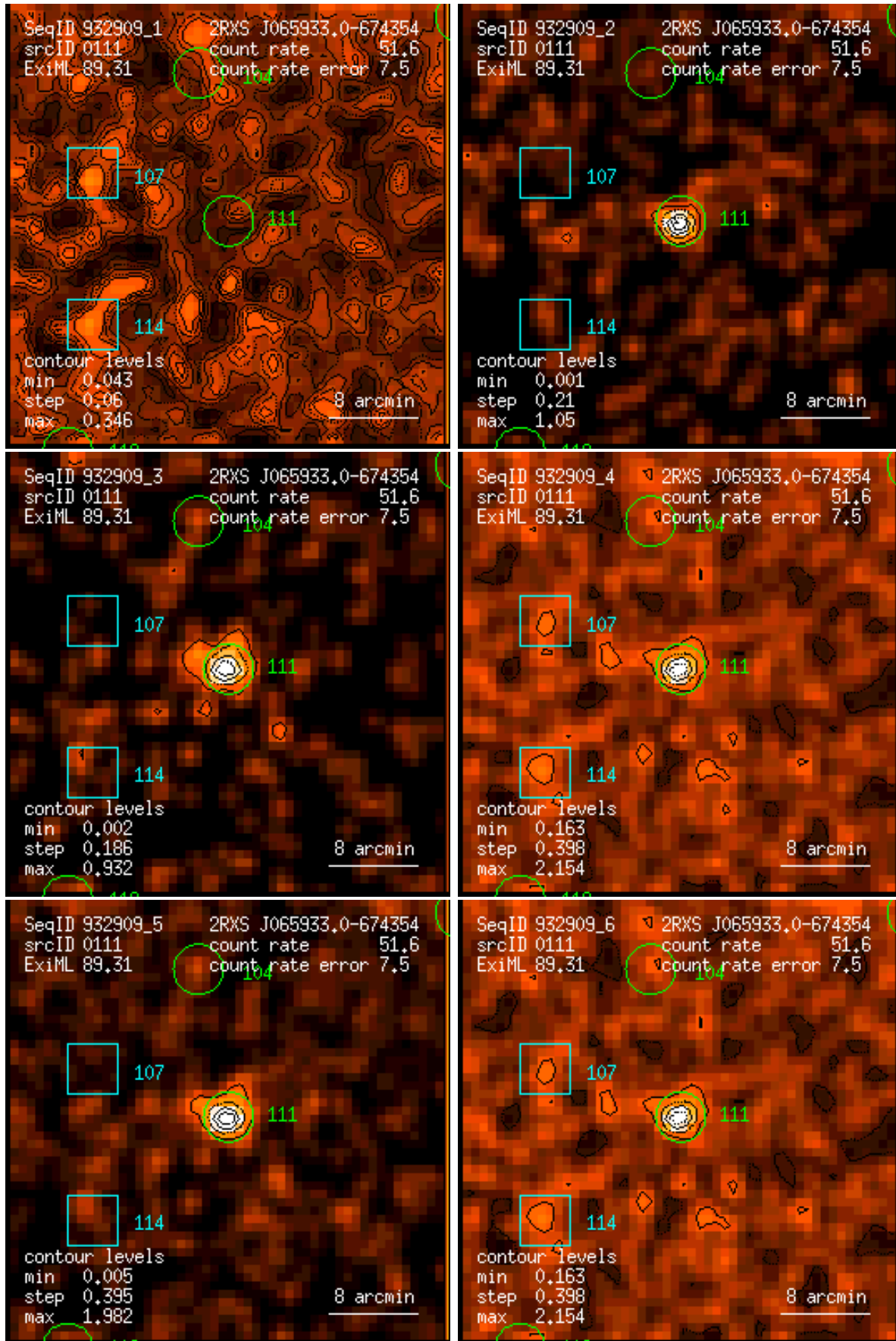
Figure 111: RASS 932909: detection 0111: band rate images, Gaussian filter: (1) PSPC channels 11 – 41, (2) 52 – 90, (3) 91 – 201, (4) 11 – 235, (5) 52 – 201, (6) 11 – 201. Broad band rates in counts/ks. Band rate contour levels in counts/ks/arcmin 2 .
