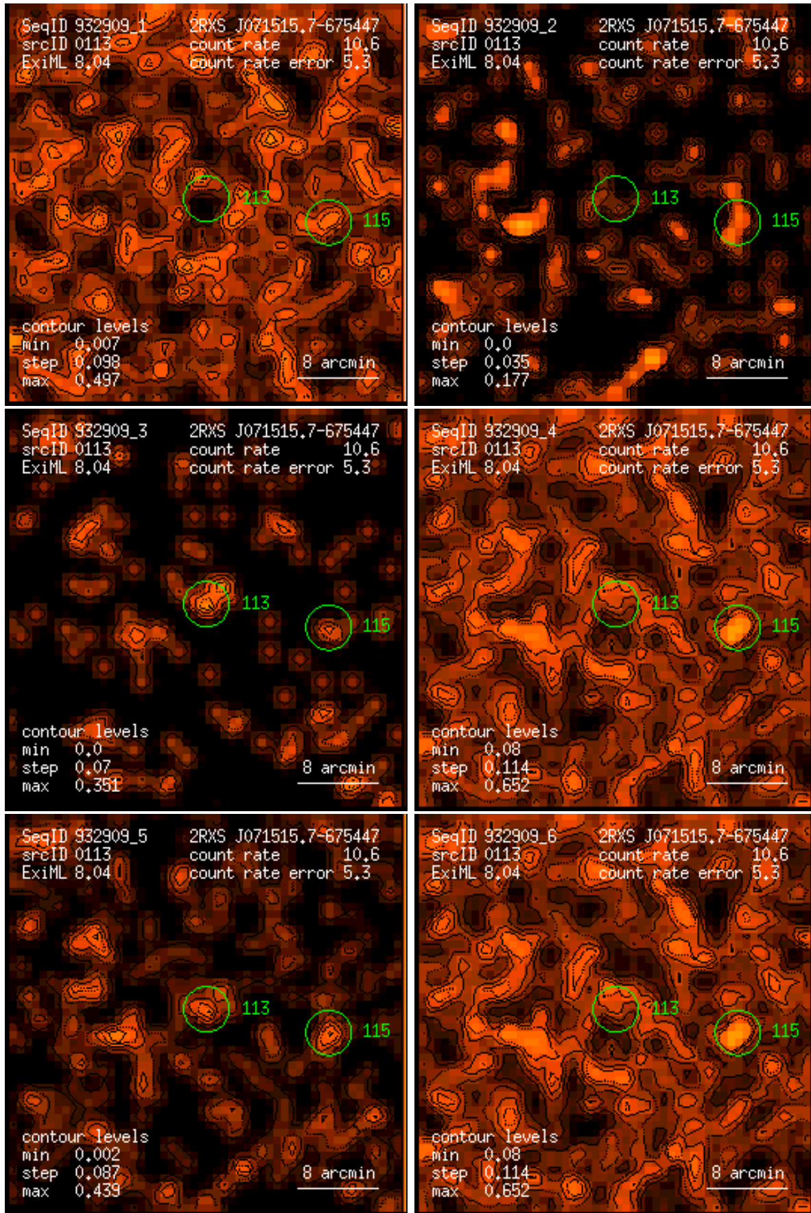
Figure 113: RASS 932909: detection 0113: band rate images, Gaussian filter: (1) PSPC channels 11 – 41, (2) 52 – 90, (3) 91 – 201, (4) 11 – 235, (5) 52 – 201, (6) 11 – 201. Broad band rates in counts/ks. Band rate contour levels in counts/ks/arcmin 2 .
