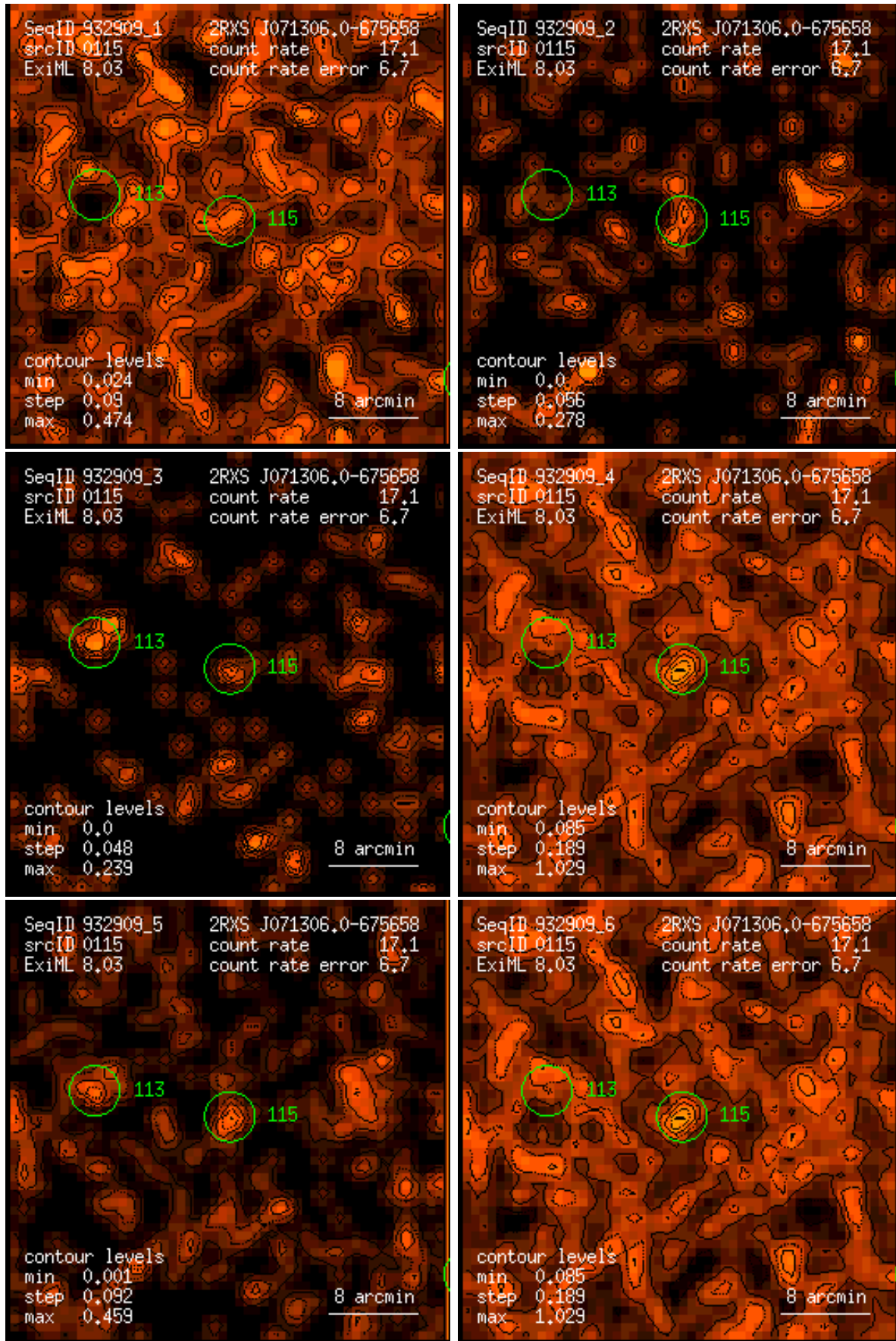
Figure 115: RASS 932909: detection 0115: band rate images, Gaussian filter: (1) PSPC channels 11 – 41, (2) 52 – 90, (3) 91 – 201, (4) 11 – 235, (5) 52 – 201, (6) 11 – 201. Broad band rates in counts/ks. Band rate contour levels in counts/ks/arcmin 2 .
