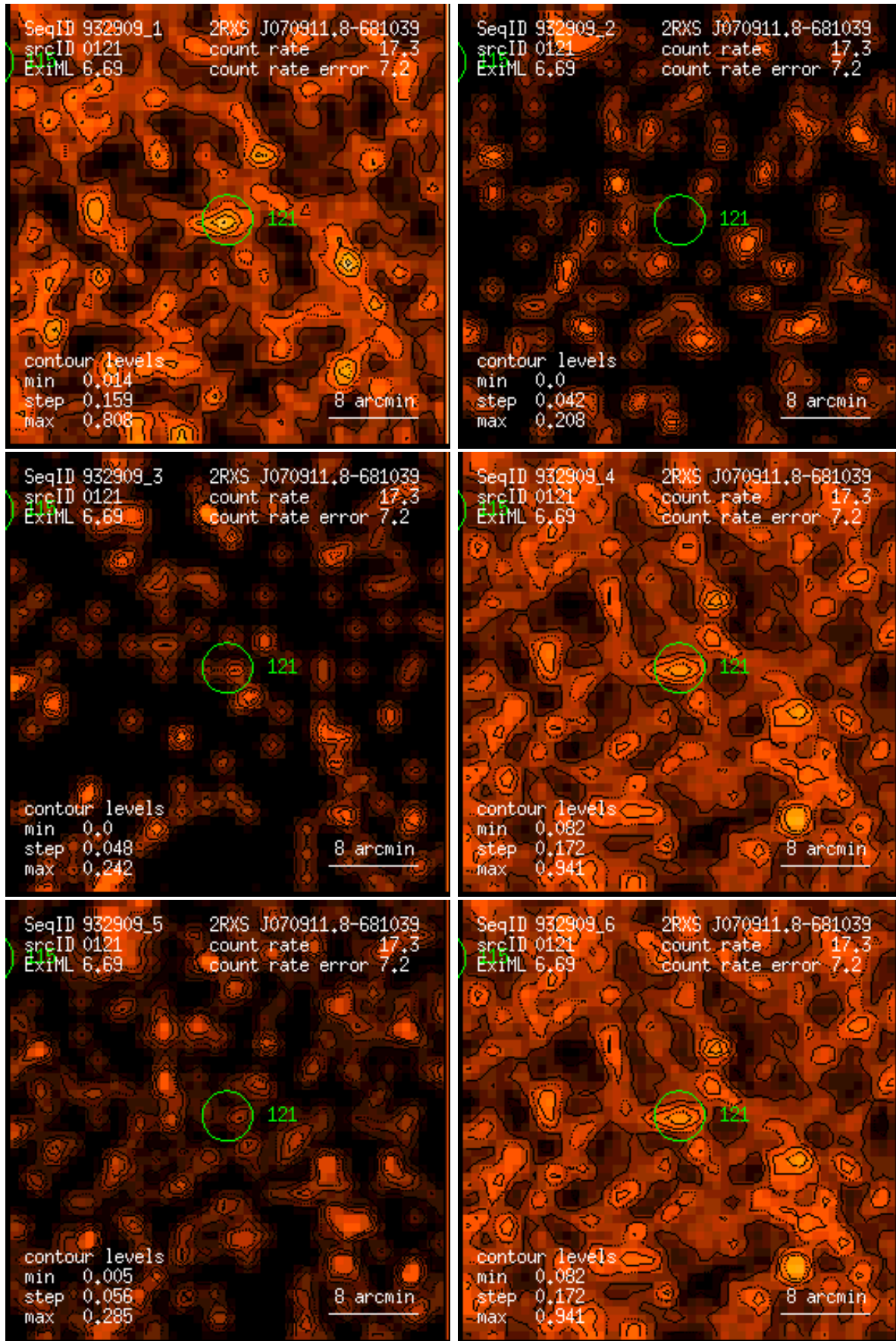
Figure 121: RASS 932909: detection 0121: band rate images, Gaussian filter: (1) PSPC channels 11 – 41, (2) 52 – 90, (3) 91 – 201, (4) 11 – 235, (5) 52 – 201, (6) 11 – 201. Broad band rates in counts/ks. Band rate contour levels in counts/ks/arcmin 2 .
