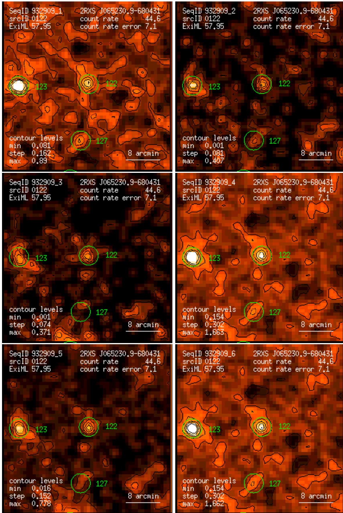
Figure 122: RASS 932909: detection 0122: band rate images, Gaussian filter: (1) PSPC channels 11 – 41, (2) 52 – 90, (3) 91 – 201, (4) 11 – 235, (5) 52 – 201, (6) 11 – 201. Broad band rates in counts/ks. Band rate contour levels in counts/ks/arcmin 2 .
