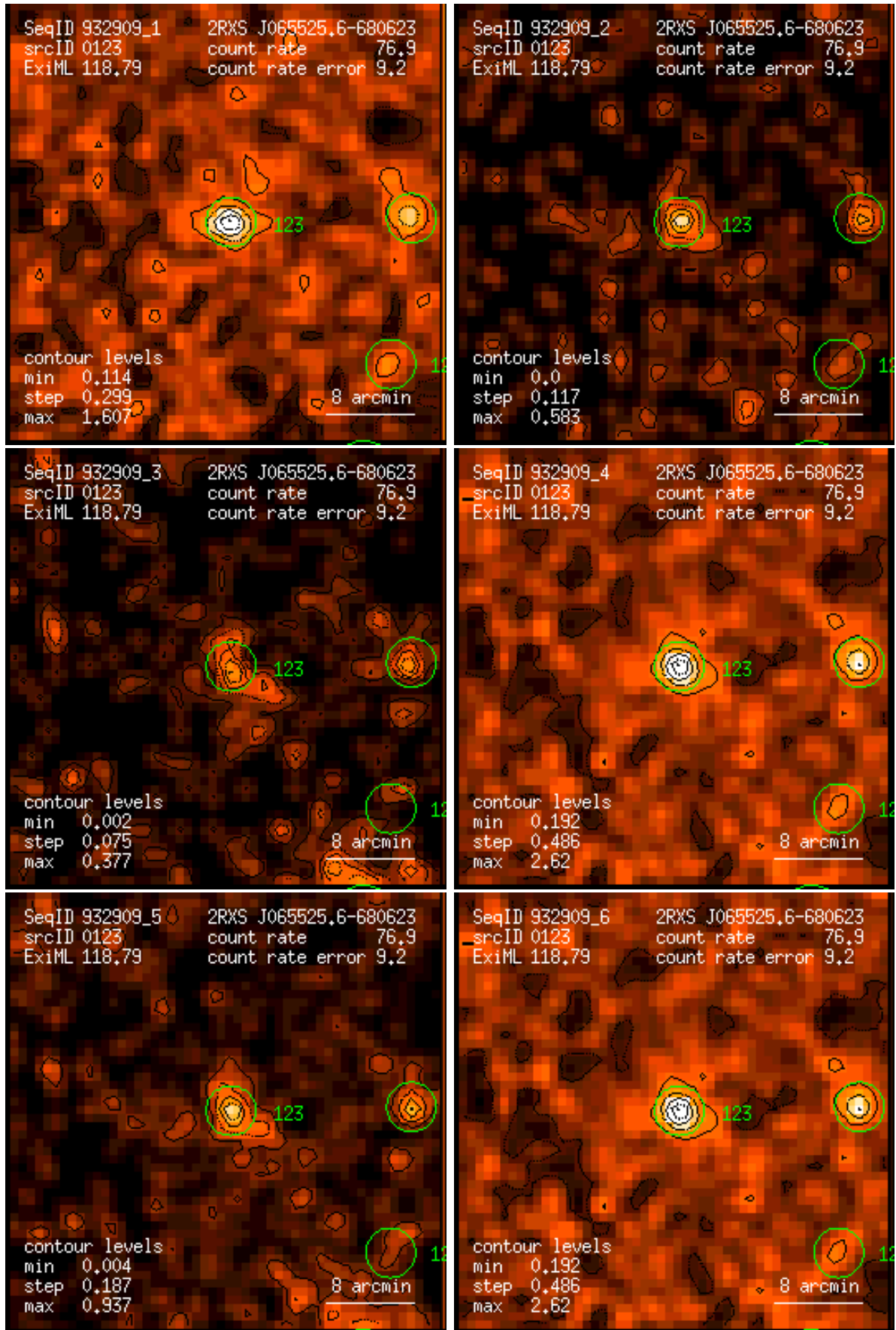
Figure 123: RASS 932909: detection 0123: band rate images, Gaussian filter: (1) PSPC channels 11 – 41, (2) 52 – 90, (3) 91 – 201, (4) 11 – 235, (5) 52 – 201, (6) 11 – 201. Broad band rates in counts/ks. Band rate contour levels in counts/ks/arcmin 2 .
