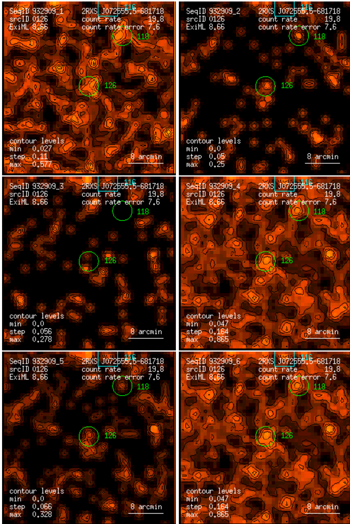
Figure 126: RASS 932909: detection 0126: band rate images, Gaussian filter: (1) PSPC channels 11 – 41, (2) 52 – 90, (3) 91 – 201, (4) 11 – 235, (5) 52 – 201, (6) 11 – 201. Broad band rates in counts/ks. Band rate contour levels in counts/ks/arcmin 2 .
