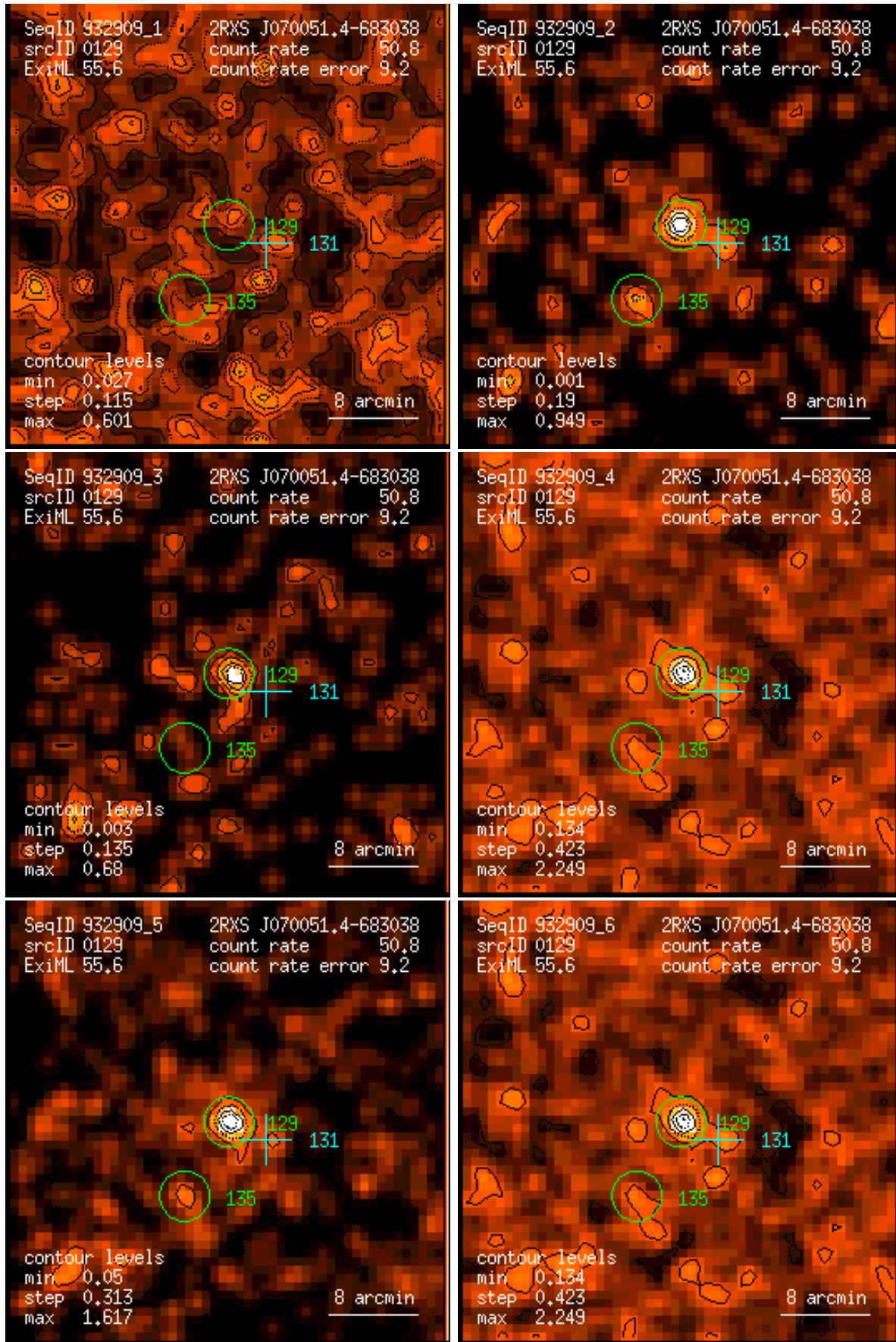
Figure 129: RASS 932909: detection 0129: band rate images, Gaussian filter: (1) PSPC channels 11 – 41, (2) 52 – 90, (3) 91 – 201, (4) 11 – 235, (5) 52 – 201, (6) 11 – 201. Broad band rates in counts/ks. Band rate contour levels in counts/ks/arcmin 2 .
