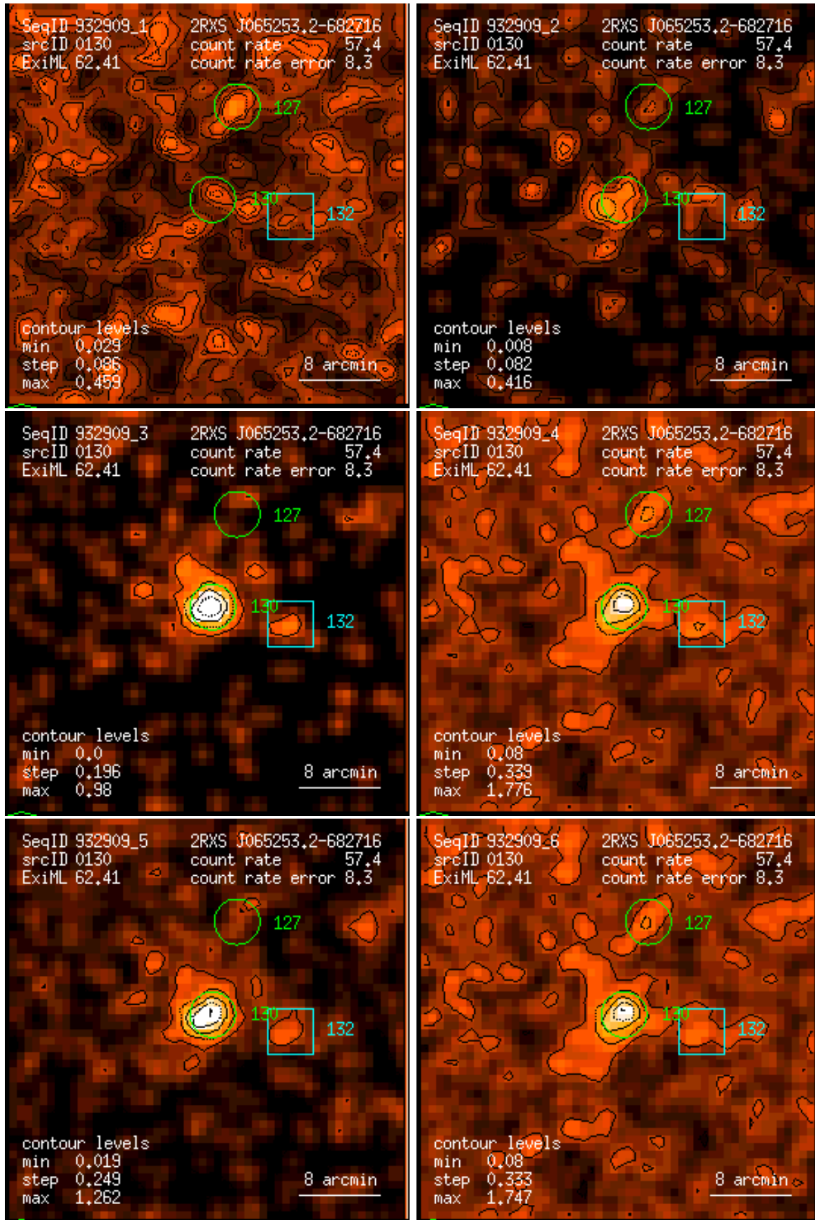
Figure 130: RASS 932909: detection 0130: band rate images, Gaussian filter: (1) PSPC channels 11 – 41, (2) 52 – 90, (3) 91 – 201, (4) 11 – 235, (5) 52 – 201, (6) 11 – 201. Broad band rates in counts/ks. Band rate contour levels in counts/ks/arcmin 2 .
