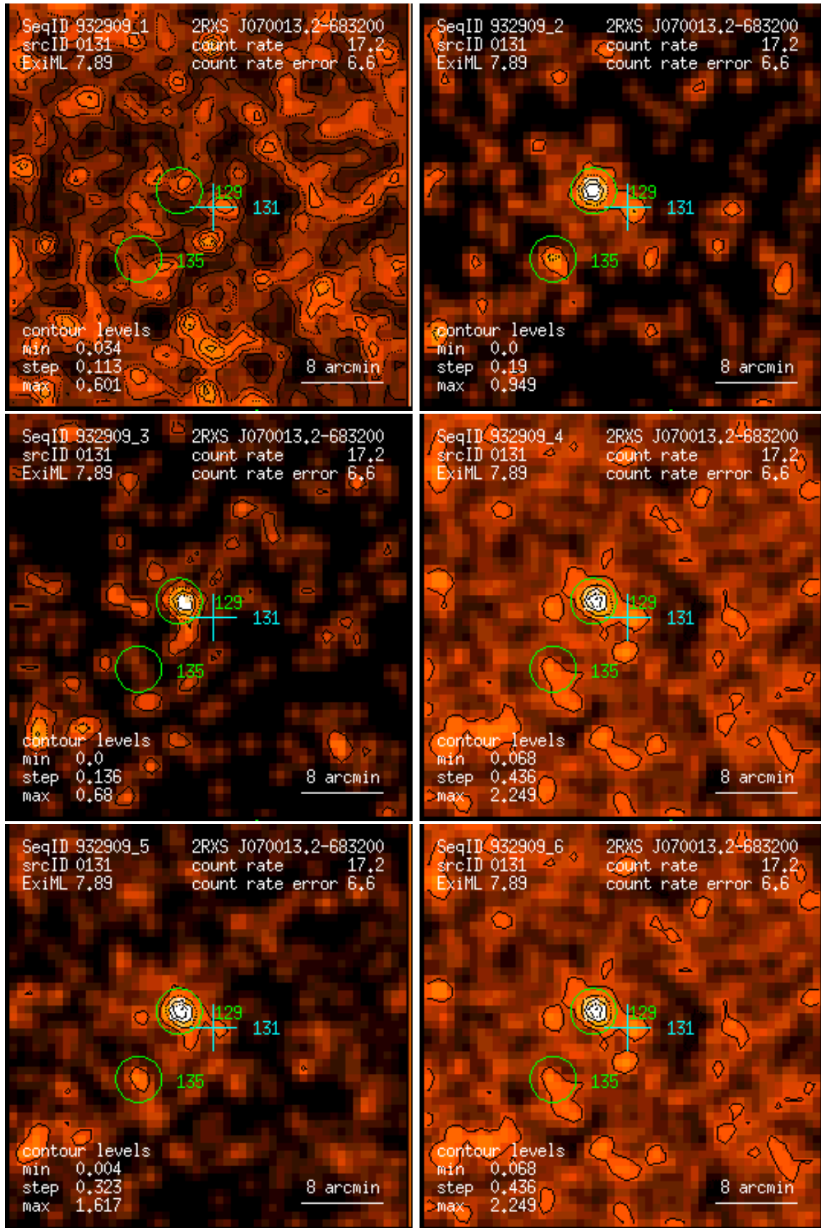
Figure 131: RASS 932909: detection 0131: band rate images, Gaussian filter: (1) PSPC channels 11 – 41, (2) 52 – 90, (3) 91 – 201, (4) 11 – 235, (5) 52 – 201, (6) 11 – 201. Broad band rates in counts/ks. Band rate contour levels in counts/ks/arcmin 2 .
