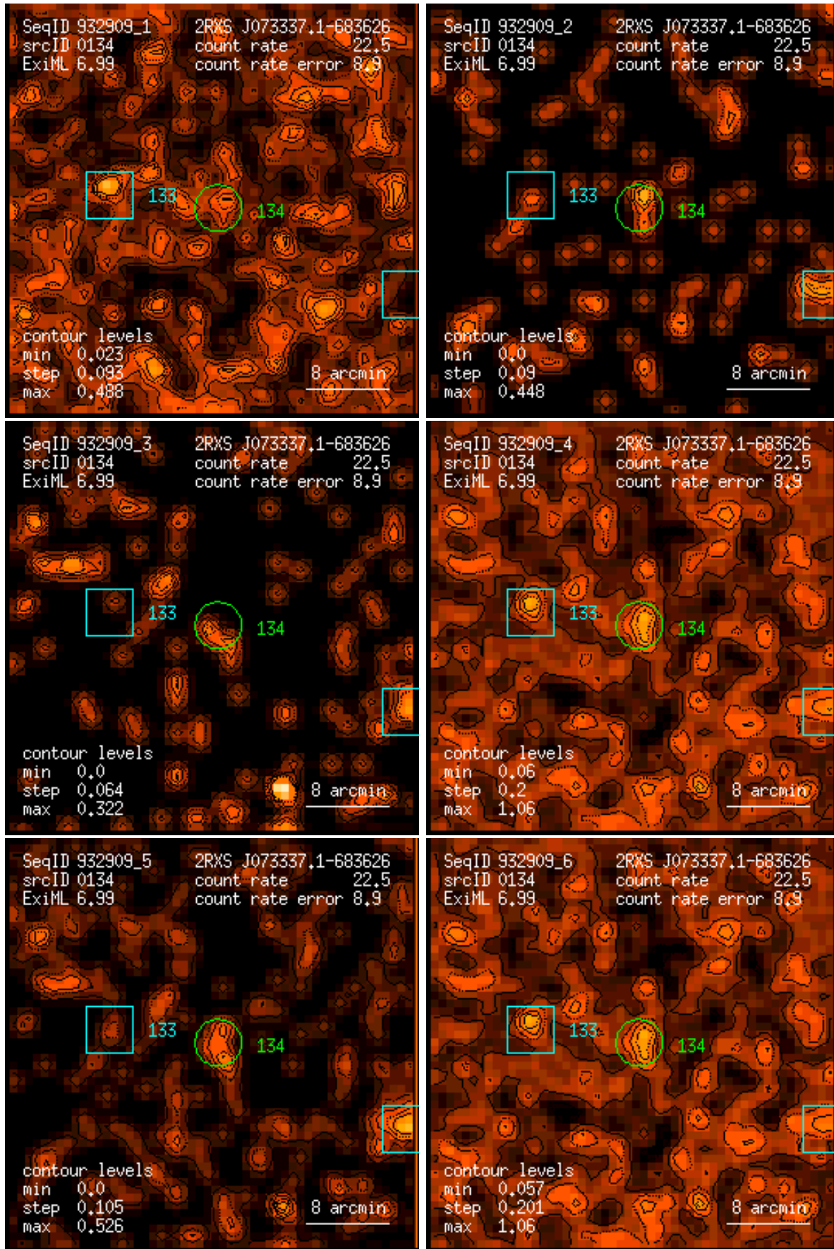
Figure 134: RASS 932909: detection 0134: band rate images, Gaussian filter: (1) PSPC channels 11 – 41, (2) 52 – 90, (3) 91 – 201, (4) 11 – 235, (5) 52 – 201, (6) 11 – 201. Broad band rates in counts/ks. Band rate contour levels in counts/ks/arcmin 2 .
