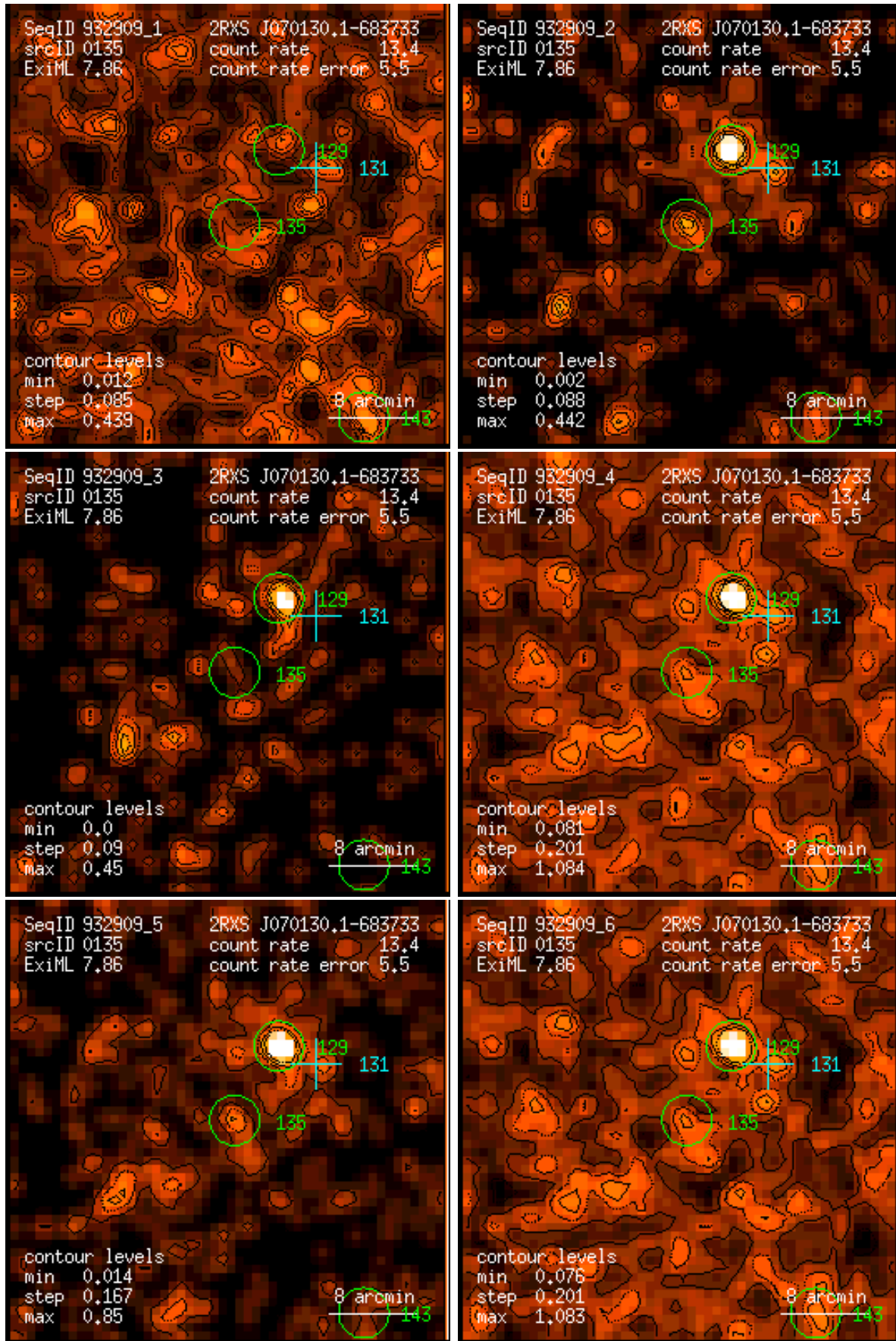
Figure 135: RASS 932909: detection 0135: band rate images, Gaussian filter: (1) PSPC channels 11 – 41, (2) 52 – 90, (3) 91 – 201, (4) 11 – 235, (5) 52 – 201, (6) 11 – 201. Broad band rates in counts/ks. Band rate contour levels in counts/ks/arcmin 2 .
