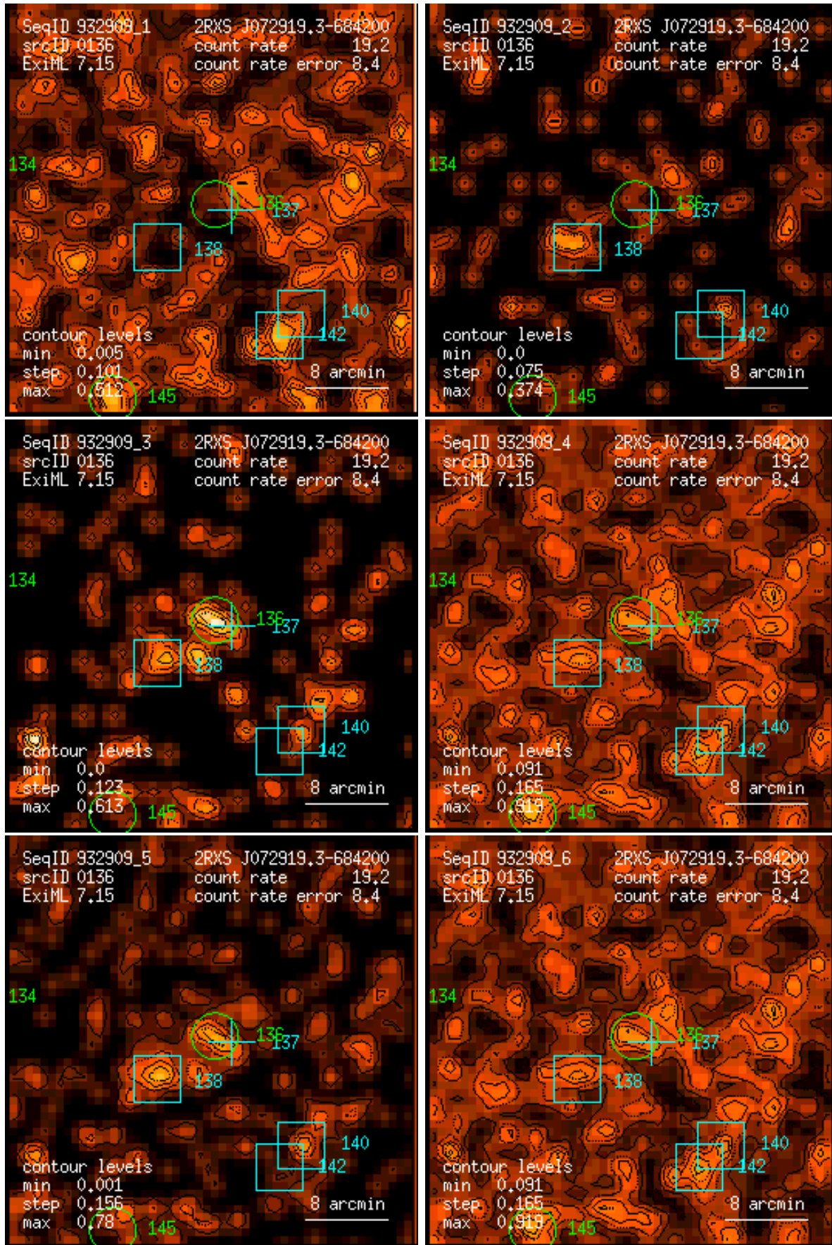
Figure 136: RASS 932909: detection 0136: band rate images, Gaussian filter: (1) PSPC channels 11 – 41, (2) 52 – 90, (3) 91 – 201, (4) 11 – 235, (5) 52 – 201, (6) 11 – 201. Broad band rates in counts/ks. Band rate contour levels in counts/ks/arcmin 2 .
