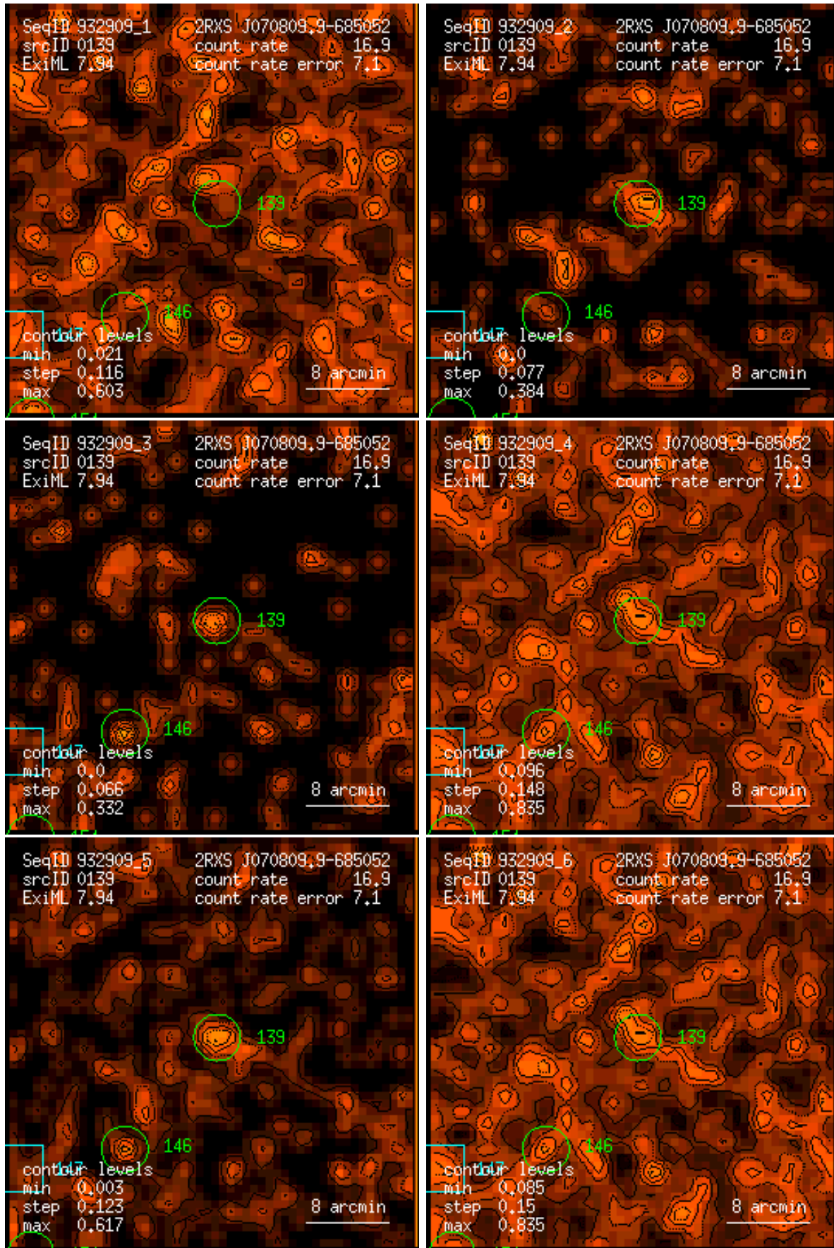
Figure 139: RASS 932909: detection 0139: band rate images, Gaussian filter: (1) PSPC channels 11 – 41, (2) 52 – 90, (3) 91 – 201, (4) 11 – 235, (5) 52 – 201, (6) 11 – 201. Broad band rates in counts/ks. Band rate contour levels in counts/ks/arcmin 2 .
