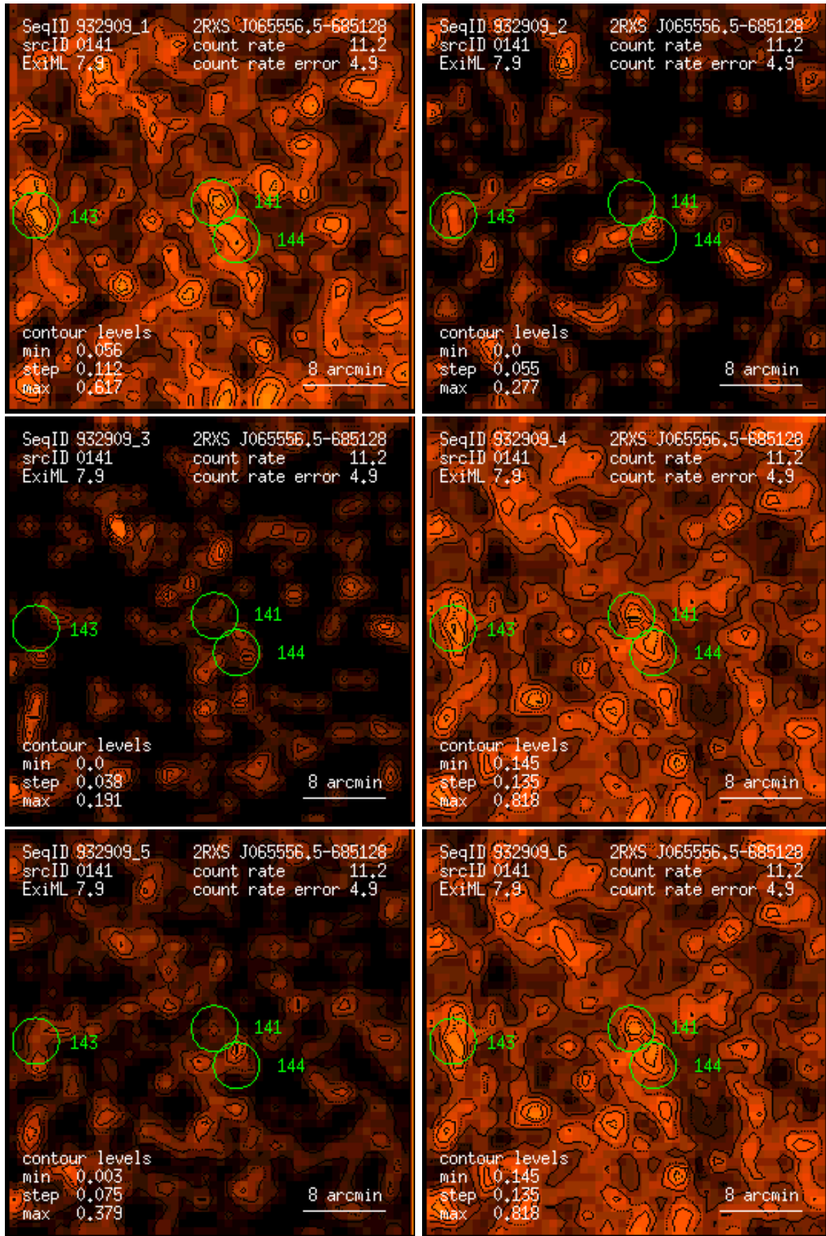
Figure 141: RASS 932909: detection 0141: band rate images, Gaussian filter: (1) PSPC channels 11 – 41, (2) 52 – 90, (3) 91 – 201, (4) 11 – 235, (5) 52 – 201, (6) 11 – 201. Broad band rates in counts/ks. Band rate contour levels in counts/ks/arcmin 2 .
