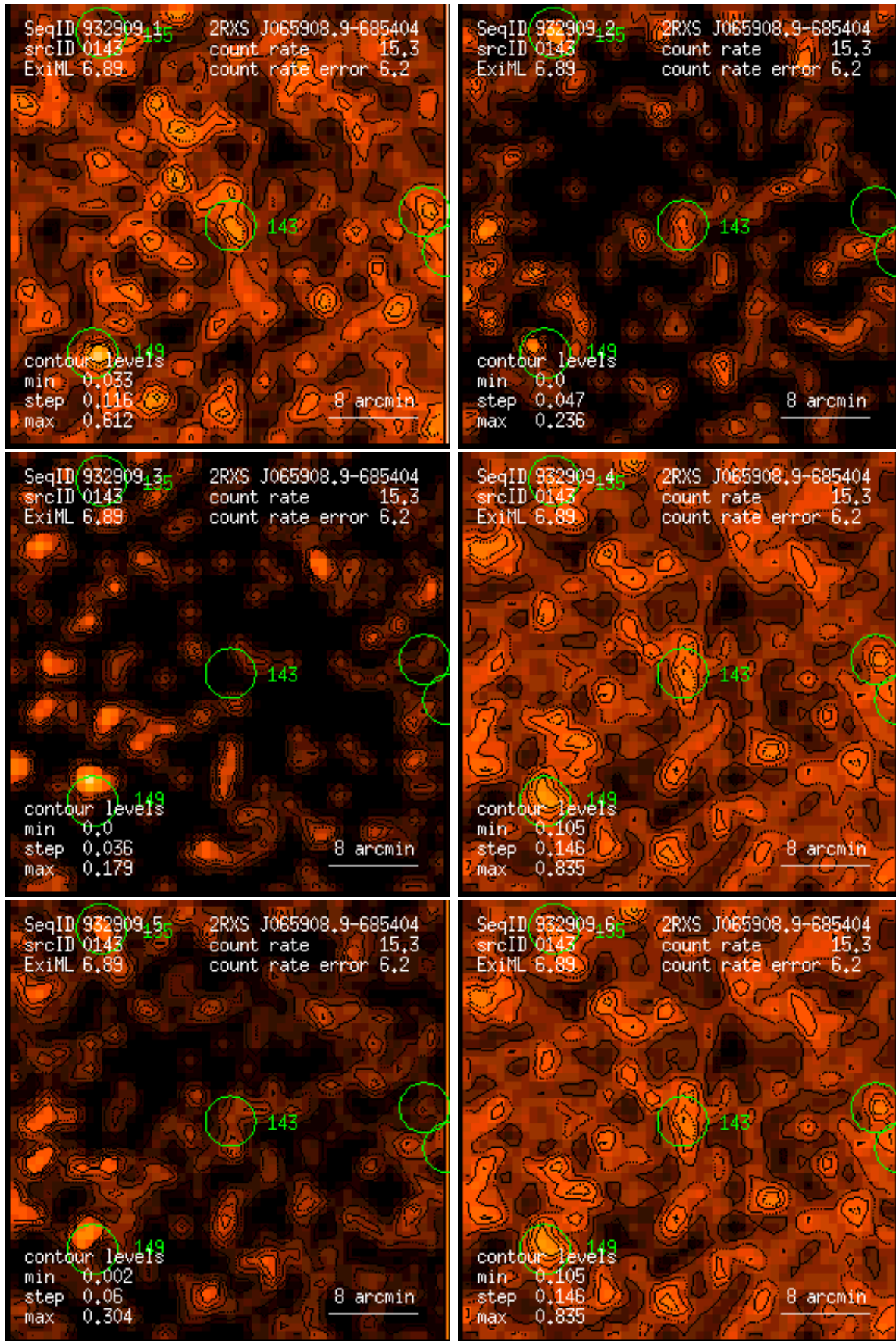
Figure 143: RASS 932909: detection 0143: band rate images, Gaussian filter: (1) PSPC channels 11 – 41, (2) 52 – 90, (3) 91 – 201, (4) 11 – 235, (5) 52 – 201, (6) 11 – 201. Broad band rates in counts/ks. Band rate contour levels in counts/ks/arcmin 2 .
