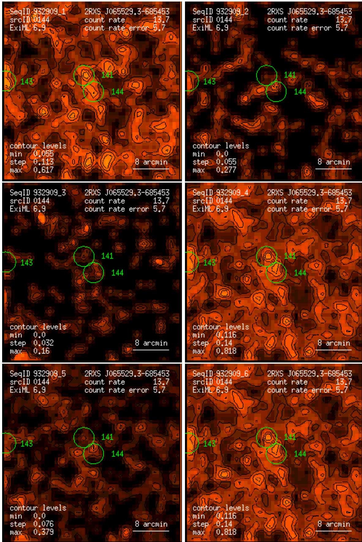
Figure 144: RASS 932909: detection 0144: band rate images, Gaussian filter: (1) PSPC channels 11 – 41, (2) 52 – 90, (3) 91 – 201, (4) 11 – 235, (5) 52 – 201, (6) 11 – 201. Broad band rates in counts/ks. Band rate contour levels in counts/ks/arcmin 2 .
