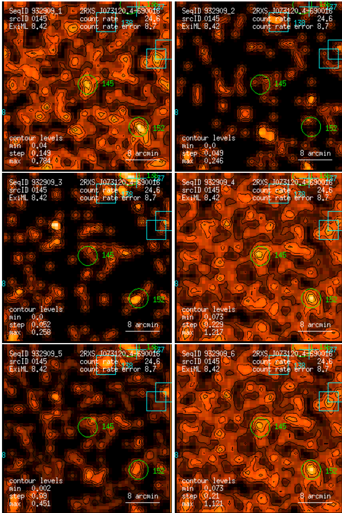
Figure 145: RASS 932909: detection 0145: band rate images, Gaussian filter: (1) PSPC channels 11 – 41, (2) 52 – 90, (3) 91 – 201, (4) 11 – 235, (5) 52 – 201, (6) 11 – 201. Broad band rates in counts/ks. Band rate contour levels in counts/ks/arcmin 2 .
