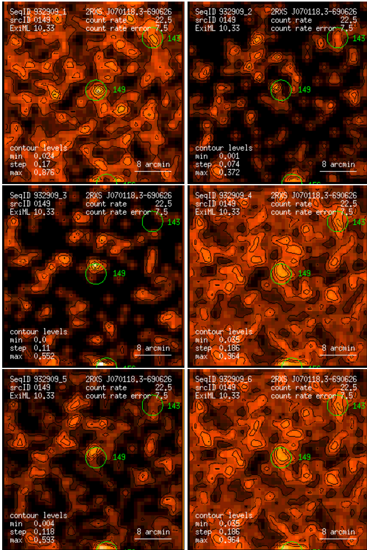
Figure 149: RASS 932909: detection 0149: band rate images, Gaussian filter: (1) PSPC channels 11 – 41, (2) 52 – 90, (3) 91 – 201, (4) 11 – 235, (5) 52 – 201, (6) 11 – 201. Broad band rates in counts/ks. Band rate contour levels in counts/ks/arcmin 2 .
