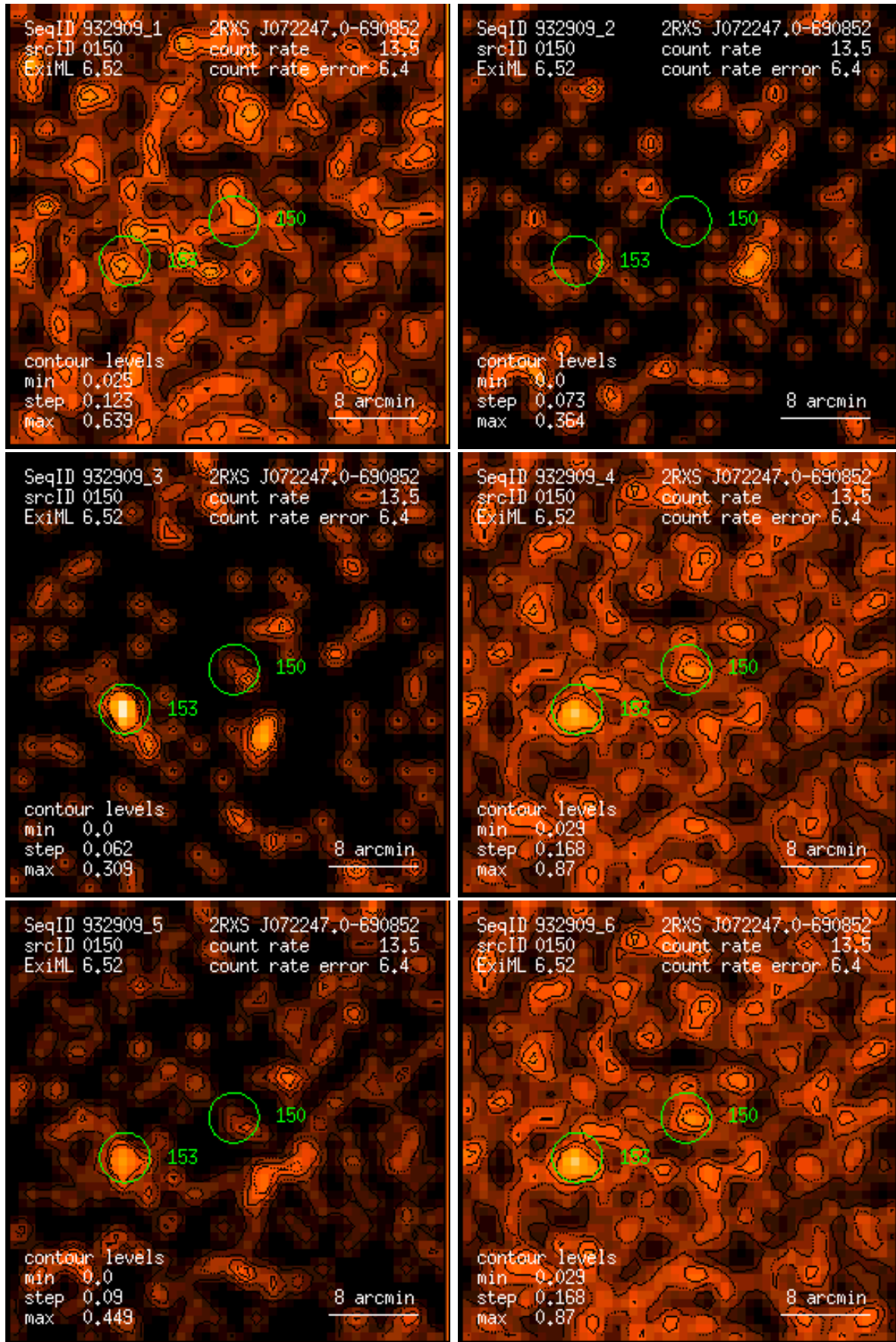
Figure 150: RASS 932909: detection 0150: band rate images, Gaussian filter: (1) PSPC channels 11 – 41, (2) 52 – 90, (3) 91 – 201, (4) 11 – 235, (5) 52 – 201, (6) 11 – 201. Broad band rates in counts/ks. Band rate contour levels in counts/ks/arcmin 2 .
