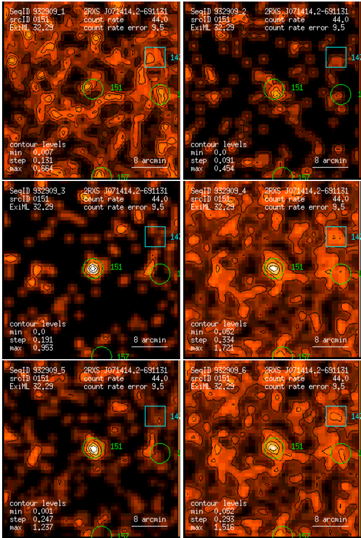
Figure 151: RASS 932909: detection 0151: band rate images, Gaussian filter: (1) PSPC channels 11 – 41, (2) 52 – 90, (3) 91 – 201, (4) 11 – 235, (5) 52 – 201, (6) 11 – 201. Broad band rates in counts/ks. Band rate contour levels in counts/ks/arcmin 2 .
