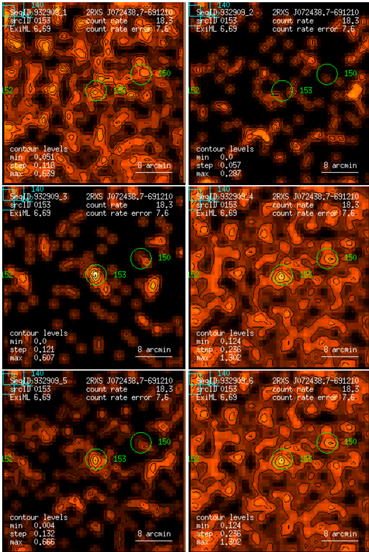
Figure 153: RASS 932909: detection 0153: band rate images, Gaussian filter: (1) PSPC channels 11 – 41, (2) 52 – 90, (3) 91 – 201, (4) 11 – 235, (5) 52 – 201, (6) 11 – 201. Broad band rates in counts/ks. Band rate contour levels in counts/ks/arcmin 2 .
