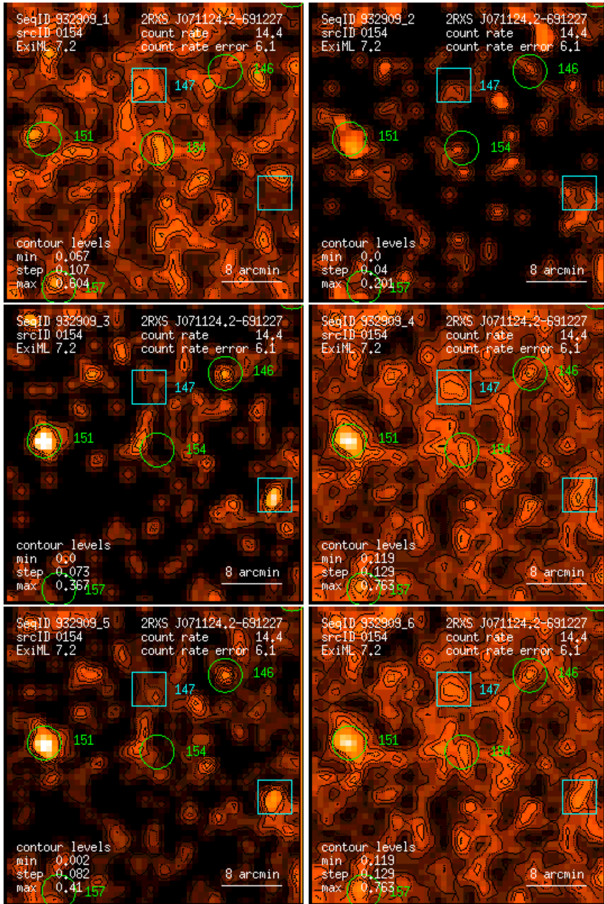
Figure 154: RASS 932909: detection 0154: band rate images, Gaussian filter: (1) PSPC channels 11 – 41, (2) 52 – 90, (3) 91 – 201, (4) 11 – 235, (5) 52 – 201, (6) 11 – 201. Broad band rates in counts/ks. Band rate contour levels in counts/ks/arcmin 2 .
