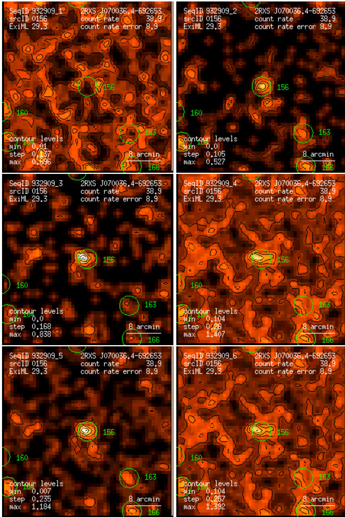
Figure 156: RASS 932909: detection 0156: band rate images, Gaussian filter: (1) PSPC channels 11 – 41, (2) 52 – 90, (3) 91 – 201, (4) 11 – 235, (5) 52 – 201, (6) 11 – 201. Broad band rates in counts/ks. Band rate contour levels in counts/ks/arcmin 2 .
