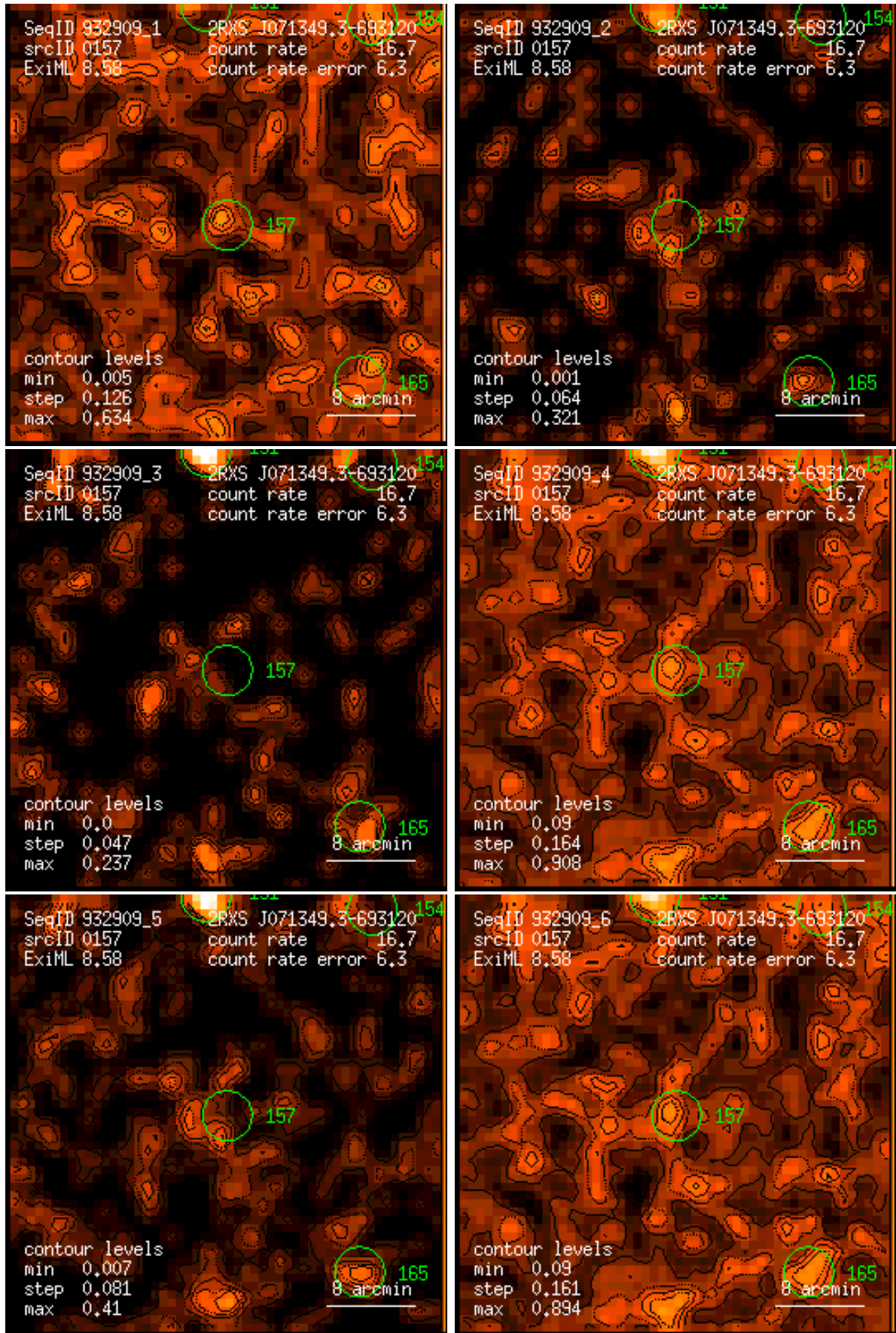
Figure 157: RASS 932909: detection 0157: band rate images, Gaussian filter: (1) PSPC channels 11 – 41, (2) 52 – 90, (3) 91 – 201, (4) 11 – 235, (5) 52 – 201, (6) 11 – 201. Broad band rates in counts/ks. Band rate contour levels in counts/ks/arcmin 2 .
