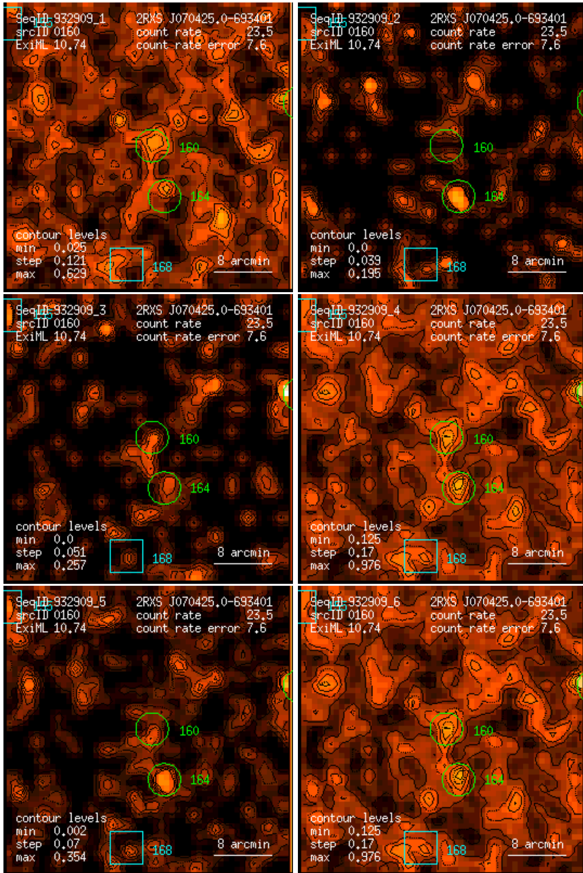
Figure 160: RASS 932909: detection 0160: band rate images, Gaussian filter: (1) PSPC channels 11 – 41, (2) 52 – 90, (3) 91 – 201, (4) 11 – 235, (5) 52 – 201, (6) 11 – 201. Broad band rates in counts/ks. Band rate contour levels in counts/ks/arcmin 2 .
